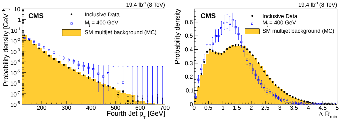
Figure 1: Probability density distributions of the fourth highest jet p_T (left) and \Delta R_{\text{min}} (right) for events from data, the simulated SM multijet sample, and a 400 GeV top squark signal. Statistical uncertainties are shown for the top squark signal as vertical bars and for data as arrows. Events contain at least four jets, each with p_T > 120 GeV and |\eta| < 2.5 , and all distributions have an area normalized to unity.
