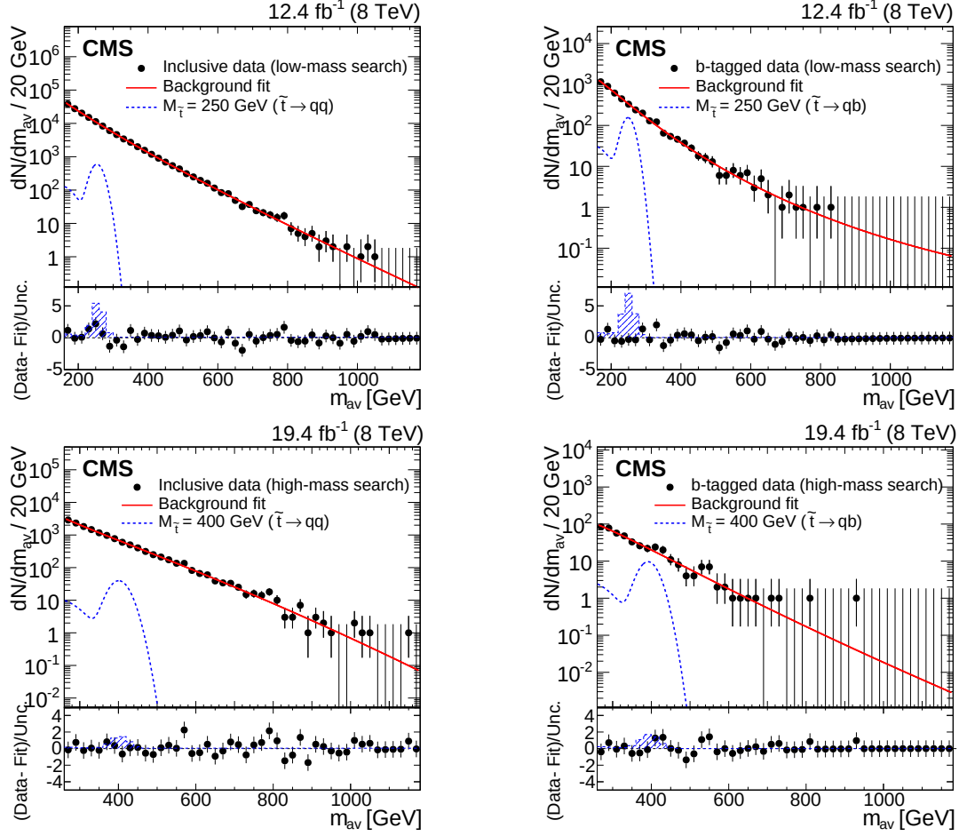
Figure 5: The m_{av} distributions with the superimposed fit from Eq. (4). The events shown satisfy requirements for the inclusive searches (left) and the heavy-flavor searches (right) in the low-mass (top) and high-mass (bottom) scenarios. The expectation for the top squark signal is indicated by the blue dashed line for the low-mass search ( M_{\tilde{t}} = 250 \text{ GeV} ) and for the high-mass search ( M_{\tilde{t}} = 400 \text{ GeV} ). The bottom part of each figure shows the difference in each bin between the data and the background estimate divided by the statistical uncertainty associated with the data, with the shaded region indicating the expected distribution in the case of the top squark signal appearing in data. The last bin in each m_{av} distribution also includes all overflow m_{av} events.
