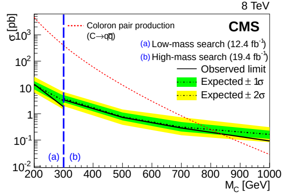
Figure 7: Observed and expected 95% CL cross section limits as a function of coloron mass for the pair-produced coloron search based on results from the low-mass (a) and high-mass (b) scenarios. The dotted red line shows the NLO+NLL predictions for coloron pair production, and the vertical dashed blue line indicates the boundary of the limits between the low- and high-mass scenarios.
