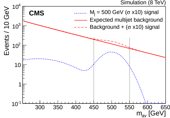
Figure 3: Distributions of the fit to simulated background SM multijet events (solid red line) and a 500 GeV top squark (dashed blue line), normalized to a factor of ten times its cross section, are shown for the high-mass optimization scenario. The dotted vertical lines represent the integration window used by the optimization procedure.
