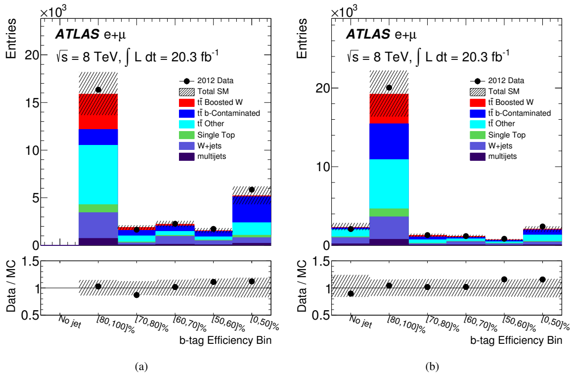
Figure 17: The efficiency-binned MV1 distribution for the (a) leading and (b) sub-leading matched small-radius in semi-leptonic t\bar{t} events. If there is no second small-radius jet with p_T > 25 GeV and \Delta R < 1 to the selected large-radius jet axis, the event is put in the ‘No jet’ category in (b). The uncertainty band includes all the experimental uncertainties on the jet p_T and jet mass and those related to the b -tagging described in Sect. 6. Statistical uncertainty bars are included on the data points but are smaller than the markers in many bins.
