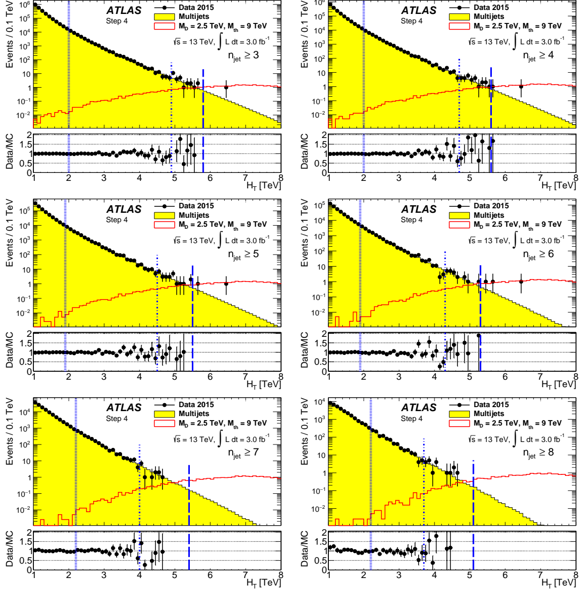
Figure 4: Data and MC simulation comparison for H_T distributions in different inclusive n_{\text{jet}} bins for the 3.0 \text{ fb}^{-1} data sample. The black hole signal with M_D = 2.5 \text{ TeV} , M_{\text{th}} = 9.0 \text{ TeV} is superimposed with the data and background MC. The MC simulation is normalized to data in the normalization region. The vertical dotted line marks the lower boundary of the control region, the vertical dashed-dotted line marks the boundary between control region and validation region, and the vertical dashed line marks the boundary between validation region and signal region. These boundaries are determined for each n_{\text{jet}} sample separately.
