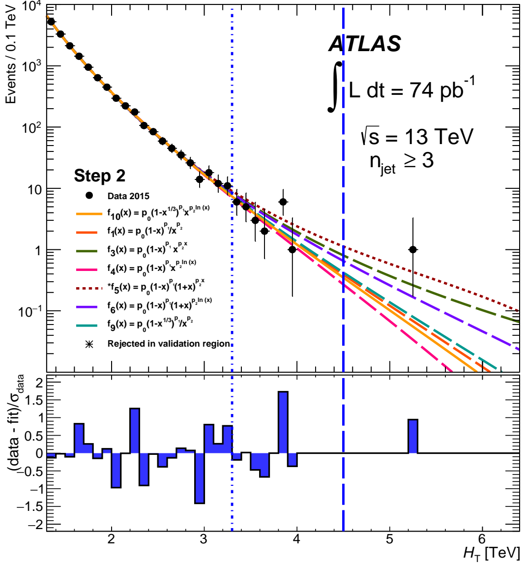
Figure 6: The data in 1.2 \text{ TeV} < H_T < 3.3 \text{ TeV} for n_{\text{jet}} \geq 3 are fitted by the baseline function (solid), and six alternative functions (dashed). The fitted functions are extrapolated to the validation region and signal region. The control, validation and signal regions are delimited by the vertical lines. The function indicated by an asterisk is rejected at 95% CL by the data in the validation region. The bottom section of the figure shows the residual significance defined as the ratio of the difference between fit and data over the statistical uncertainty of data, where the fit prediction is taken from the baseline function.
