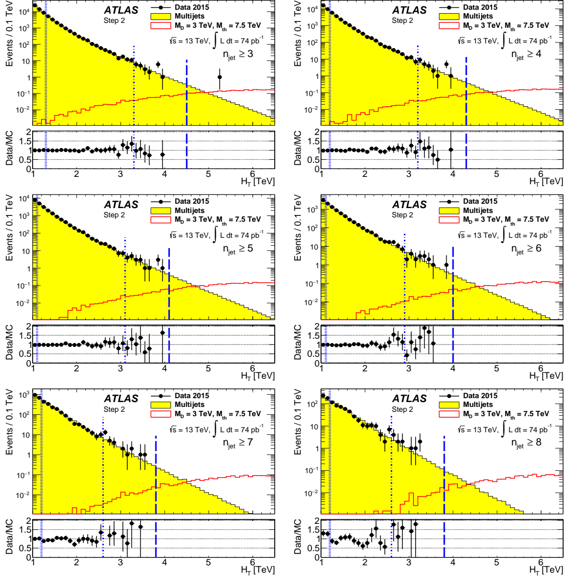
Figure 2: Data and MC simulation comparison for H_T distributions in different inclusive n_{\text{jets}} bins for the 74 \text{ pb}^{-1} data sample. The black hole signal with M_D = 3 \text{ TeV} , M_{\text{th}} = 7.5 \text{ TeV} is superimposed with the data and background MC. The MC simulation was normalized to data in the normalization region. The vertical dotted line marks the lower boundary of the control region, the vertical dashed-dotted line marks the boundary between control region and validation region, and the vertical dashed line marks the boundary between validation region and signal region. These boundaries are determined for each n_{\text{jets}} sample separately.
