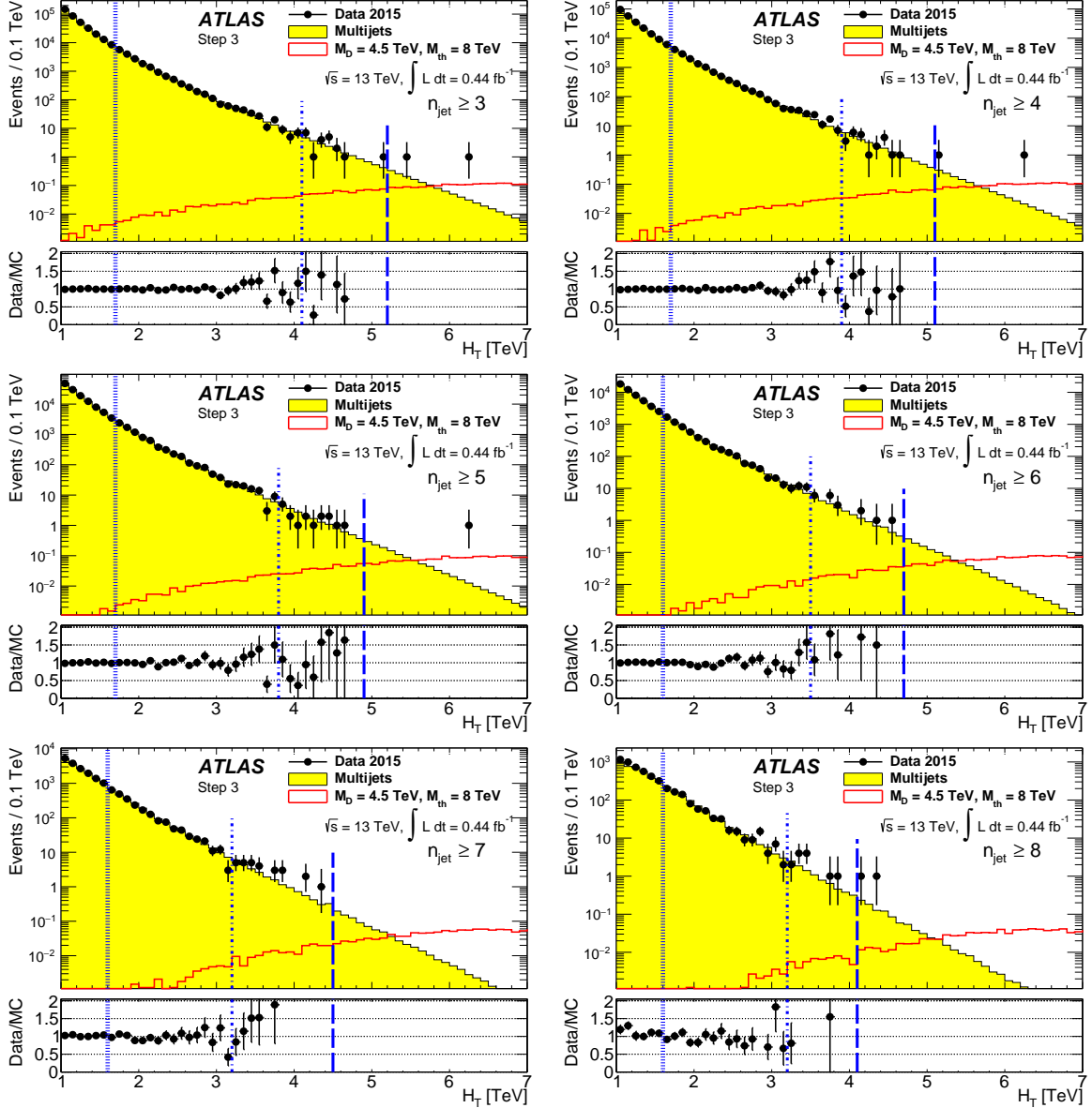
Figure 3: Data and MC simulation comparison for H_T distributions in different inclusive n_{\text{jets}} bins for the 0.44 \text{ fb}^{-1} data sample. The black hole signal with M_D = 4.5 \text{ TeV} , M_{\text{th}} = 8 \text{ TeV} is superimposed with the data and background MC. The MC simulation is normalized to data in the normalization region. The vertical dotted line marks the lower boundary of the control region, the vertical dashed-dotted line marks the boundary between control region and validation region, and the vertical dashed line marks the boundary between validation region and signal region. These boundaries are determined for each n_{\text{jets}} sample separately.
