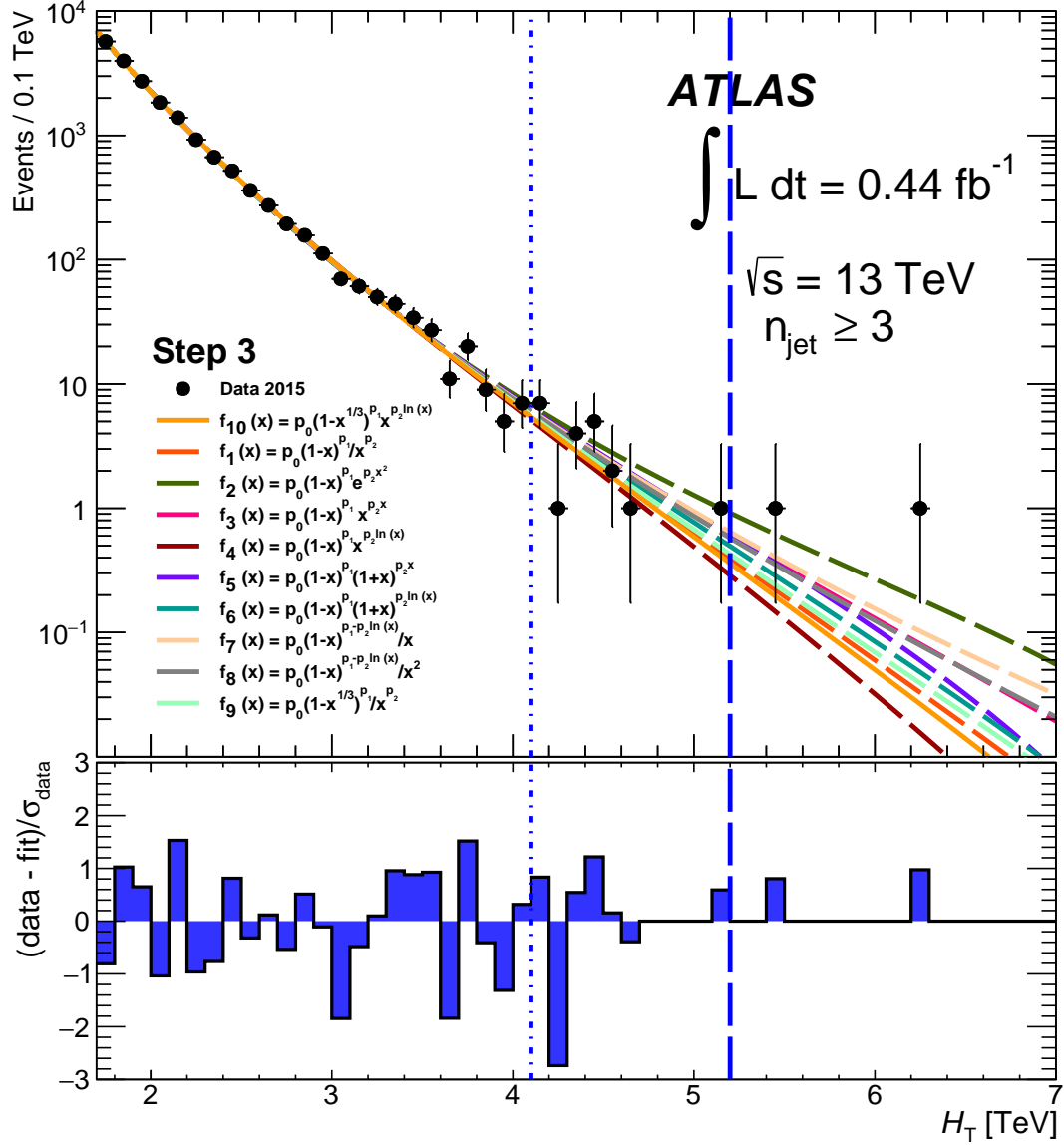
Figure 7: The data in 1.7 \text{ TeV} < H_T < 4.1 \text{ TeV} for n_{\text{jet}} \geq 3 are fitted by the baseline function (solid), and nine alternative functions (dashed). The fitted functions are extrapolated to the validation region and signal region. The control, validation and signal regions are delimited by the vertical lines. The bottom section of the figure shows the residual significance defined as the ratio of the difference between fit and data over the statistical uncertainty of data, where the fit prediction is taken from the baseline function.
