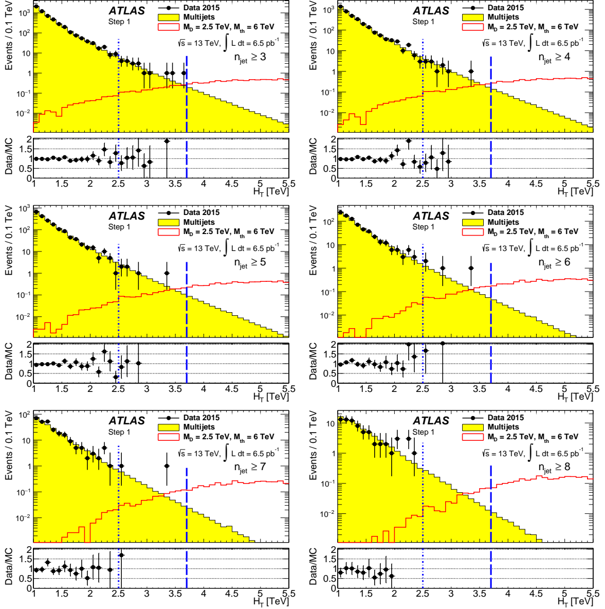
Figure 1: Data and MC simulation comparison for the distributions of the scalar sum of jet transverse momenta H_T in different inclusive n_{\text{jet}} bins for the 6.5 \text{ pb}^{-1} data sample. The black hole signal with M_D = 2.5 \text{ TeV} , M_{\text{th}} = 6.0 \text{ TeV} is superimposed with the data and background MC simulation sample. The MC is normalized to data in the normalization region. The vertical dashed-dotted line marks the boundary between control region and validation region, and the dashed line marks the boundary between validation region and signal region. The boundaries shown correspond to those determined for the n_{\text{jet}} \geq 3 case.
