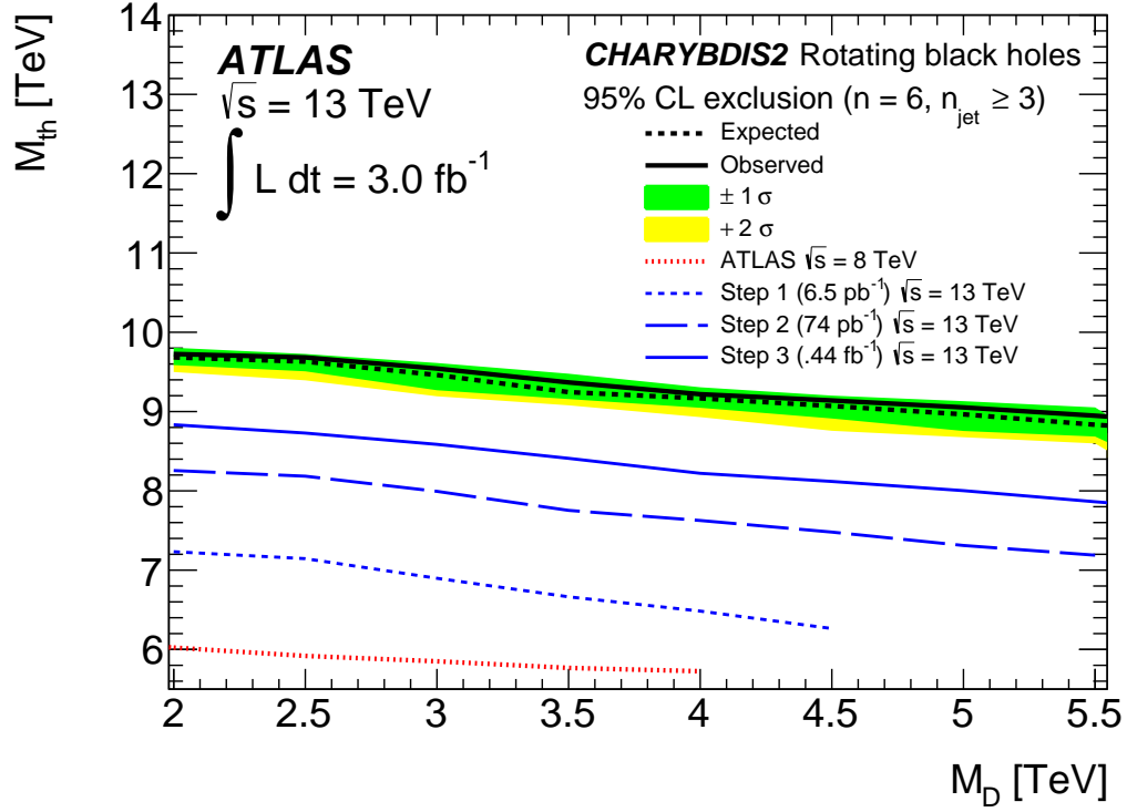
Figure 10: "The observed and expected limits on rotating black holes with n = 6 in the M_D - M_{th} grid, from the analysis with an integrated luminosity of 3.0 \text{ fb}^{-1} . The 95% CL expected limit is shown as the black dashed line, and limits corresponding to the \pm 1 \sigma and + 2 \sigma variations of the background expectation are shown as the green and yellow bands, respectively. The 95% CL observed limit is shown as the black solid line. The -2 \sigma band is not shown as it almost completely overlaps with the -1 \sigma band. The blue dashed lines corresponds to the observed limits from the first, second and third step analyses. The red dotted line corresponds to the limit from Run-1 ATLAS multijet search [5].
