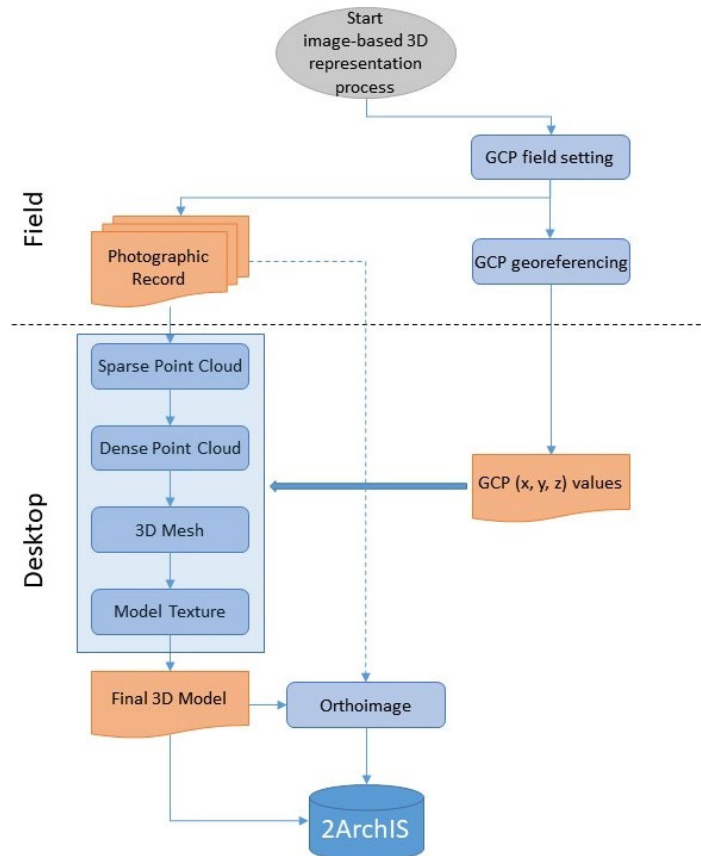
Figure 2: Simplified workflow of the 3D reconstruction process
