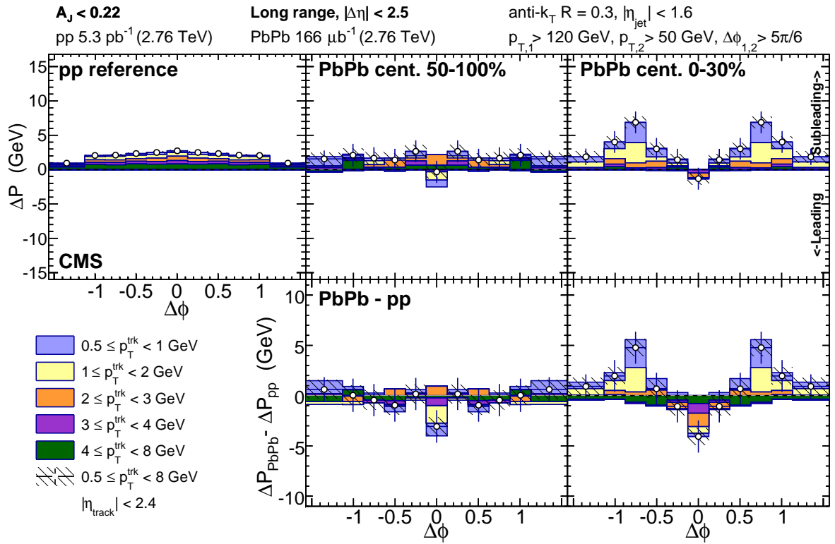
Figure 8: Top row: long-range distribution in \Delta\phi of excess p_T^{\text{trk}} in the subleading relative to leading sides for balanced dijet events with A_J < 0.22 . Bottom row: PbPb–pp difference in these \Delta\phi long-range momentum distributions. Statistical uncertainties are shown with vertical bars, and systematic uncertainties are shown with shaded boxes.
