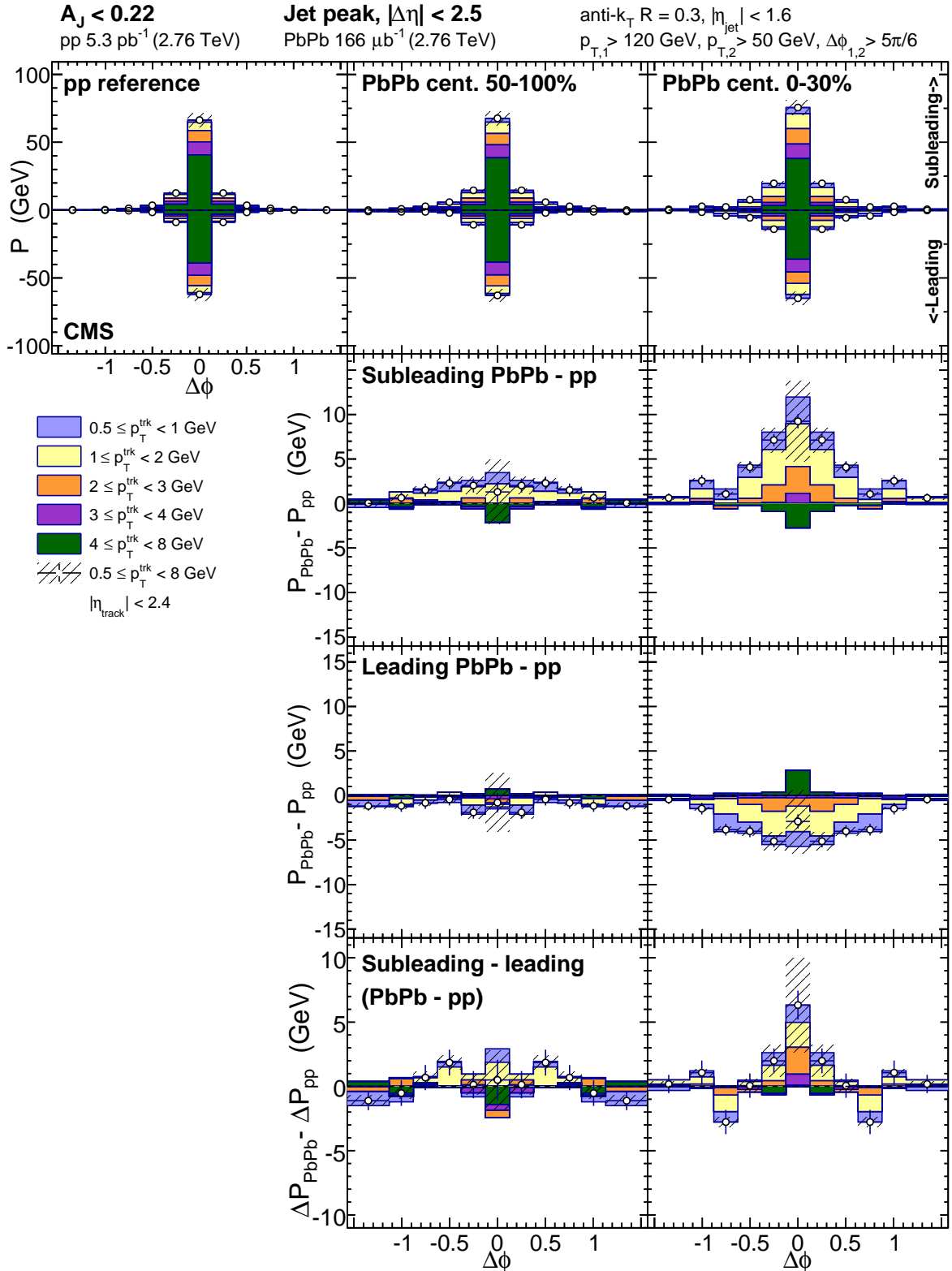
Figure 6: Top row: jet-peak (long-range subtracted) distribution in \Delta\phi of p_T^{\text{trk}} about the sub-leading (plotted positive) and leading (plotted negative) jets for balanced dijet events with A_J < 0.22 . Middle rows: PbPb–pp momentum distribution differences for subleading and leading jets. Bottom row: PbPb–pp, subleading–leading double difference in these \Delta\phi momentum distributions. Statistical uncertainties are shown with vertical bars, and systematic uncertainties are shown with shaded boxes.
