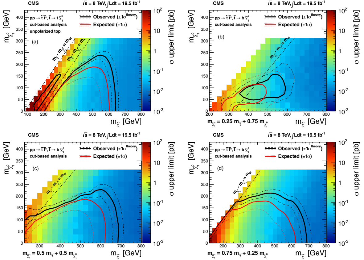
Figure 20: Interpretations based on the results of the cut-based analysis. (a) \tilde{t} \rightarrow t\tilde{\chi}_1^0 model; (b) \tilde{t} \rightarrow b\tilde{\chi}^+ model with x = 0.25 ; (c) \tilde{t} \rightarrow b\tilde{\chi}^+ model with x = 0.50 ; (d) \tilde{t} \rightarrow b\tilde{\chi}^+ model with x = 0.75 ; The color scale indicates the observed cross section upper limit. The observed (solid black), median expected (solid red), and \pm 1\sigma expected (dotted red) 95% CL exclusion contours are indicated. The variations in the excluded region due to \pm 1\sigma uncertainty of the theoretical prediction of the cross section for top-squark pair production are also indicated.
