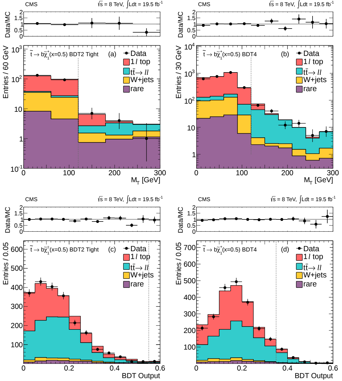
Figure 17: Comparison of data and MC simulation for the distributions of BDT output and M_T corresponding to the x = 0.5 \tilde{t} \rightarrow b\tilde{\chi}_1^+ scenario in training regions 2 and 4. The M_T distributions are shown after the requirement on the BDT output, and the BDT output distributions are shown after the M_T > 120 GeV requirement (these requirements are also indicated by vertical dashed lines on the respective distributions). (a) M_T after the tight cut on the BDT2 output; (b) M_T after the cut on the BDT4 output; (c) BDT2 output after the M_T cut; (d) BDT4 output after the M_T cut. In all distributions the last bin contains the overflow.
