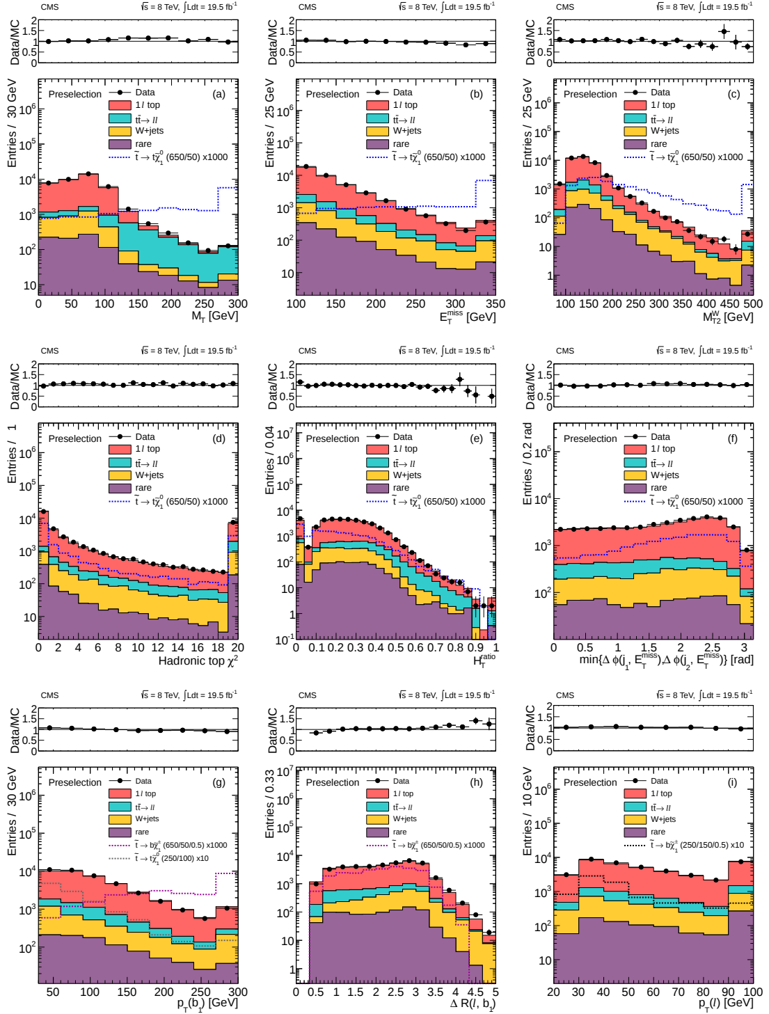
Figure 2: Comparison of data with MC simulation for the distributions of (a) M_T , (b) E_T^{\text{miss}} , (c) M_{T2}^W , (d) hadronic top \chi^2 , (e) H_T^{\text{ratio}} , (f) minimum \Delta\phi between the E_T^{\text{miss}} vector and the two leading jets, (g) p_T of the leading b-tagged jet, (h) \Delta R between the leading b-tagged jet and the lepton, and (i) lepton p_T , after the preselection. For the plots (a)-(f), distributions for the \tilde{t} \rightarrow t\tilde{\chi}_1^0 model with m_{\tilde{t}} = 650 GeV and m_{\tilde{\chi}_1^0} = 50 GeV, scaled by a factor of 1000, are overlaid. We also show distributions of \tilde{t} \rightarrow t\tilde{\chi}_1^0 with m_{\tilde{t}} = 250 GeV and m_{\tilde{\chi}_1^0} = 100 GeV for (g), scaled by 10, and of \tilde{t} \rightarrow b\tilde{\chi}_1^+ with m_{\tilde{t}} = 650 GeV, m_{\tilde{\chi}_1^+} = 50 GeV, and x = 0.5 for (h) and (i), scaled by 1000, as well as of m_{\tilde{t}} = 250 GeV, m_{\tilde{\chi}_1^0} = 150 GeV, and x = 0.5 for (i), scaled by 10. In all distributions the last bin contains the overflow.
