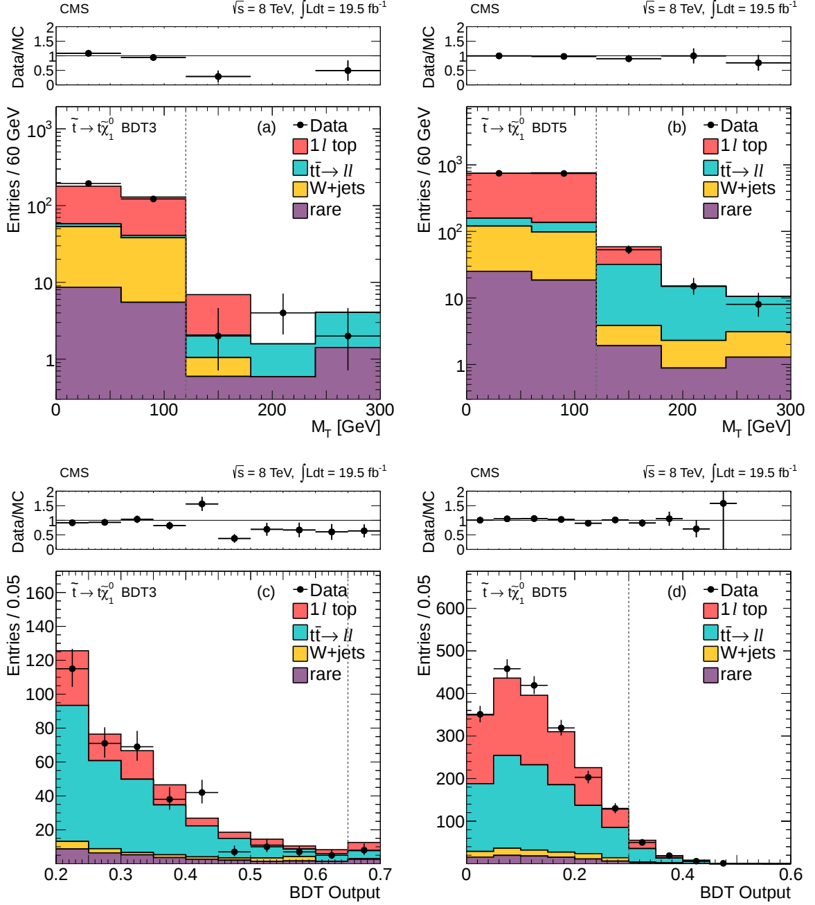
Figure 14: Comparison of data and MC simulation for the distributions of BDT output and M_T corresponding to the \tilde{t} \rightarrow \tilde{t}\chi_1^0 scenario in training regions 3 and 5. The M_T distributions are shown after the requirement on the BDT output, and the BDT output distributions are shown after the M_T > 120 GeV requirement (these requirements are also indicated by vertical dashed lines on the respective distributions). (a) M_T after the cut on the BDT3 output; (b) M_T after the cut on the BDT5 output; (c) BDT3 output after the M_T cut; (d) BDT5 output after the M_T cut. In all distributions the last bin contains the overflow.
