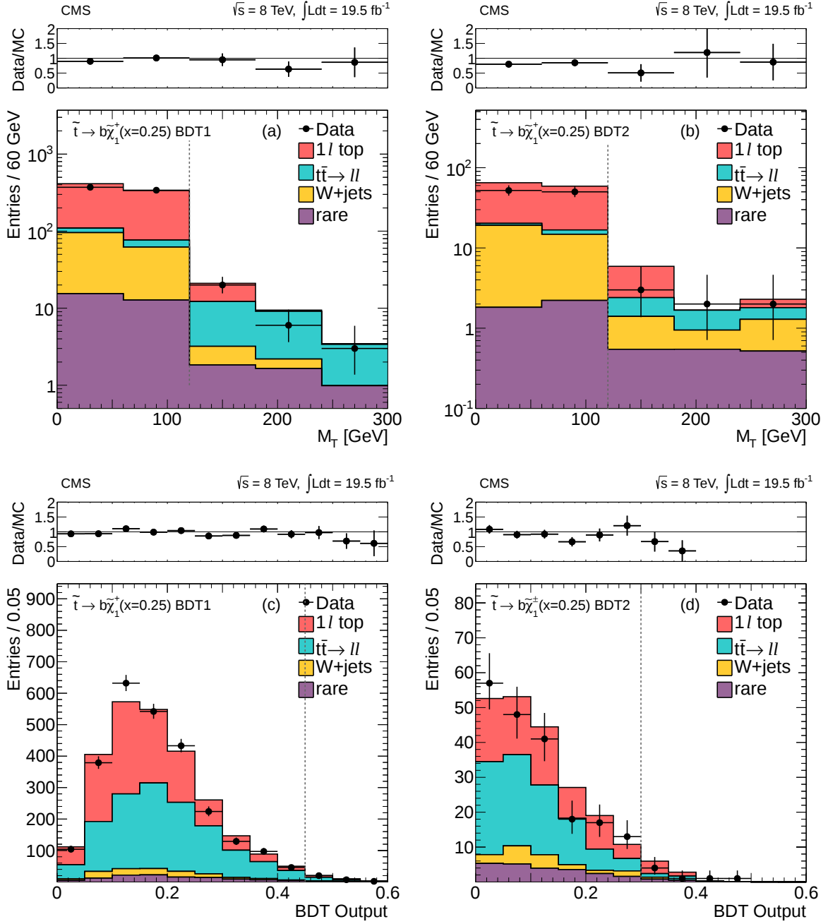
Figure 15: Comparison of data and MC simulation for the distributions of BDT output and M_T corresponding to the x = 0.25 \tilde{t} \rightarrow b\tilde{\chi}_1^+ scenario in training regions 1 and 2. The M_T distributions are shown after the requirement on the BDT output, and the BDT output distributions are shown after the M_T > 120 GeV requirement (these requirements are also indicated by vertical dashed lines on the respective distributions). (a) M_T after the cut on the BDT1 output; (b) M_T after the cut on the BDT2 output; (c) BDT1 output after the M_T cut; (d) BDT2 output after the M_T cut. In all distributions the last bin contains the overflow.
