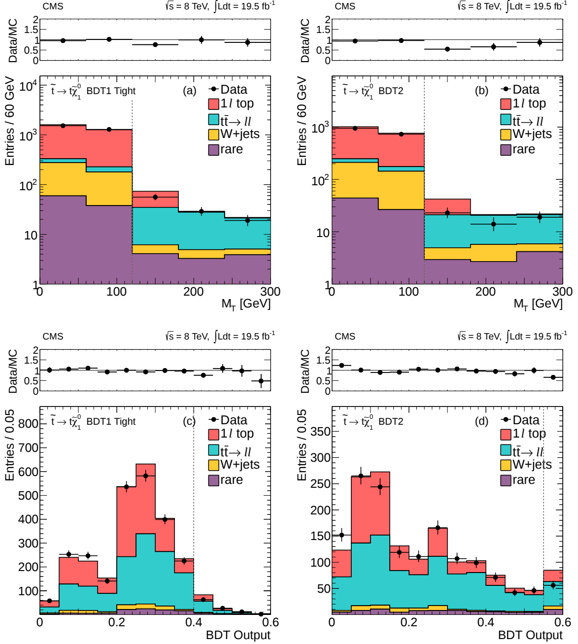
Figure 13: Comparison of data and MC simulation for the distributions of BDT output and M_T corresponding to the \tilde{t} \rightarrow t\tilde{\chi}_1^0 scenario in training regions 1 and 2. The M_T distributions are shown after the requirement on the BDT output, and the BDT output distributions are shown after the M_T > 120 \text{ GeV} requirement (these requirements are also indicated by vertical dashed lines on the respective distributions). (a) M_T after the tight cut on the BDT1 output; (b) M_T after the cut on the BDT2 output; (c) BDT1 output after the M_T cut; (d) BDT2 output after the M_T cut. In all distributions the last bin contains the overflow.
