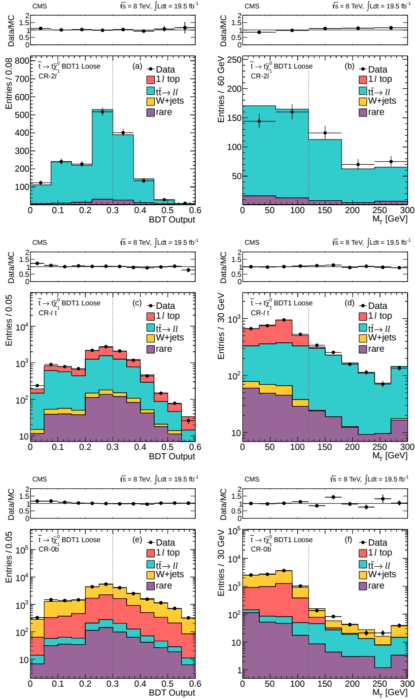
Figure 6: Comparison of data and MC simulation for the distributions of M_T and BDT output for the control regions associated with the BDT trained in region 1 for the \tilde{t} \rightarrow t\tilde{\chi}_1^0 scenario. The M_T distributions are shown after the “BDT1 loose” requirement indicated by vertical dashed lines on the BDT output plots. (a)-(b): CR-2l; (c)-(d): CR-lt; (e)-(f): CR-0b. The vertical dashed lines in the M_T plots correspond to the M_T > 120 GeV selection requirement. For CR-0b, the scale factors are applied to the MC distribution in the M_T tail. The last bin in all distributions contains the overflow.
