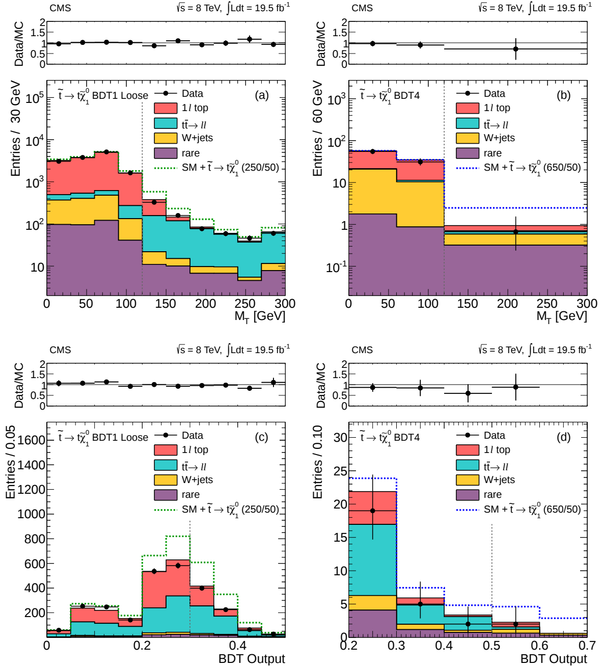
Figure 8: Comparison of data and MC simulation for the distributions of BDT output and M_T corresponding to the tightest and loosest signal region selections in the \tilde{t} \rightarrow t\tilde{\chi}_1^0 scenario. The M_T distributions are shown after the requirement on the BDT output, and the BDT output distributions are shown after the M_T > 120 GeV requirement (these requirements are also indicated by vertical dashed lines on the respective distributions). (a) M_T after the loose cut on the BDT1 output; (b) M_T after the cut on the BDT4 output; (c) BDT1 output after the M_T cut; (d) BDT4 output after the M_T cut. Expected signal distributions for m_{\tilde{\chi}_1^0} = 50 GeV and m_{\tilde{t}} = 250 GeV or 650 GeV are also overlayed, as indicated in the figures. In plot (b), the bin to the right of the vertical line contains all events with M_T > 120 GeV, and has been scaled by a factor of 1/3 to indicate the number of events per 60 GeV. In all distributions the last bin contains the overflow.
