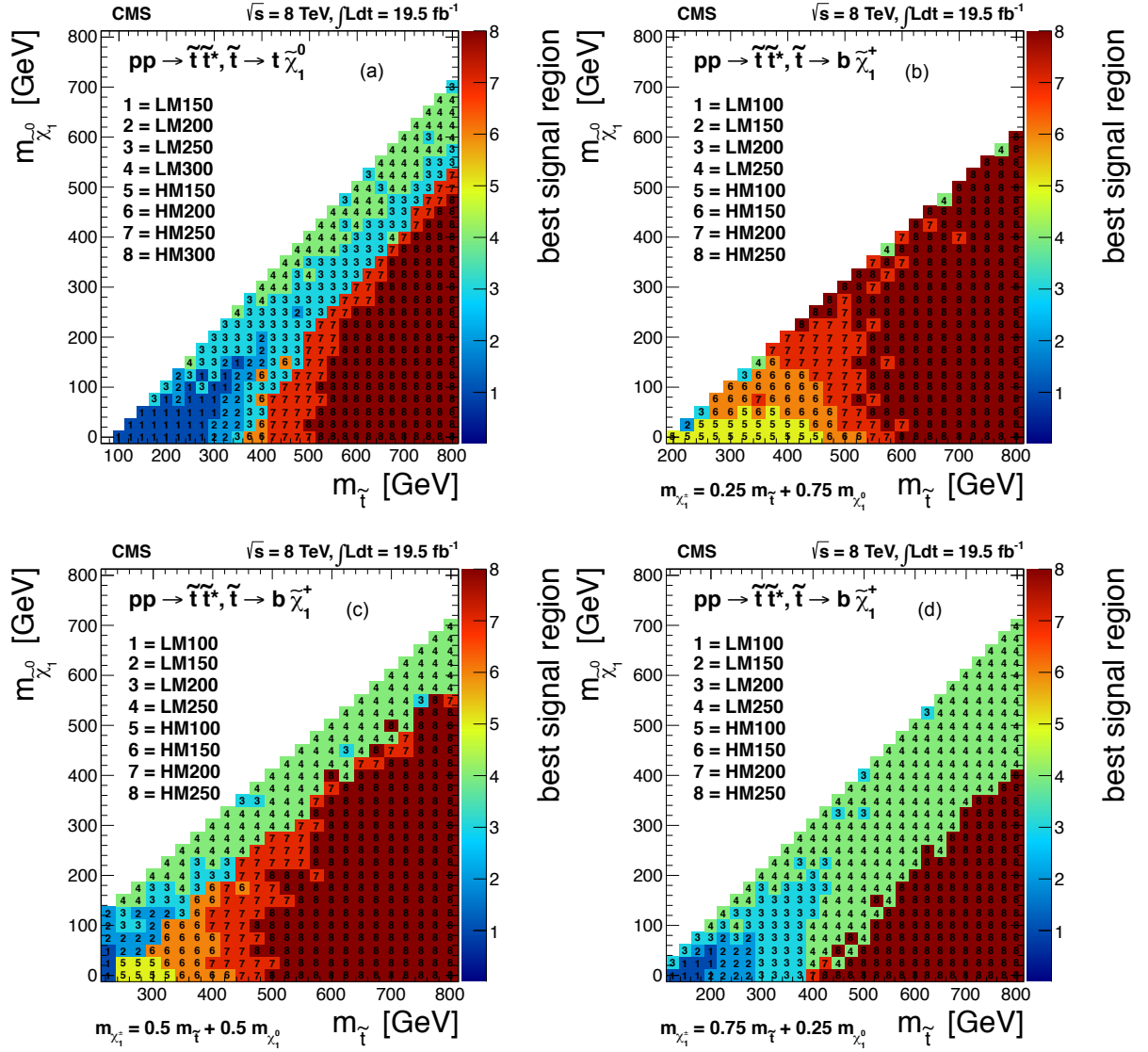
Figure 22: The most sensitive signal region in the m_{\tilde{\chi}_1^0} vs. m_{\tilde{t}} parameter space in the cut-based analysis, for the (a) \tilde{t} \rightarrow t\tilde{\chi}_1^0 model, and the \tilde{t} \rightarrow b\tilde{\chi}_1^+ model with chargino mass parameter (b) x = 0.25 , (c) 0.5 , and (d) 0.75 . LM and HM refer to low \Delta M and high \Delta M , respectively, and the number indicates the E_T^{\text{miss}} requirement.
