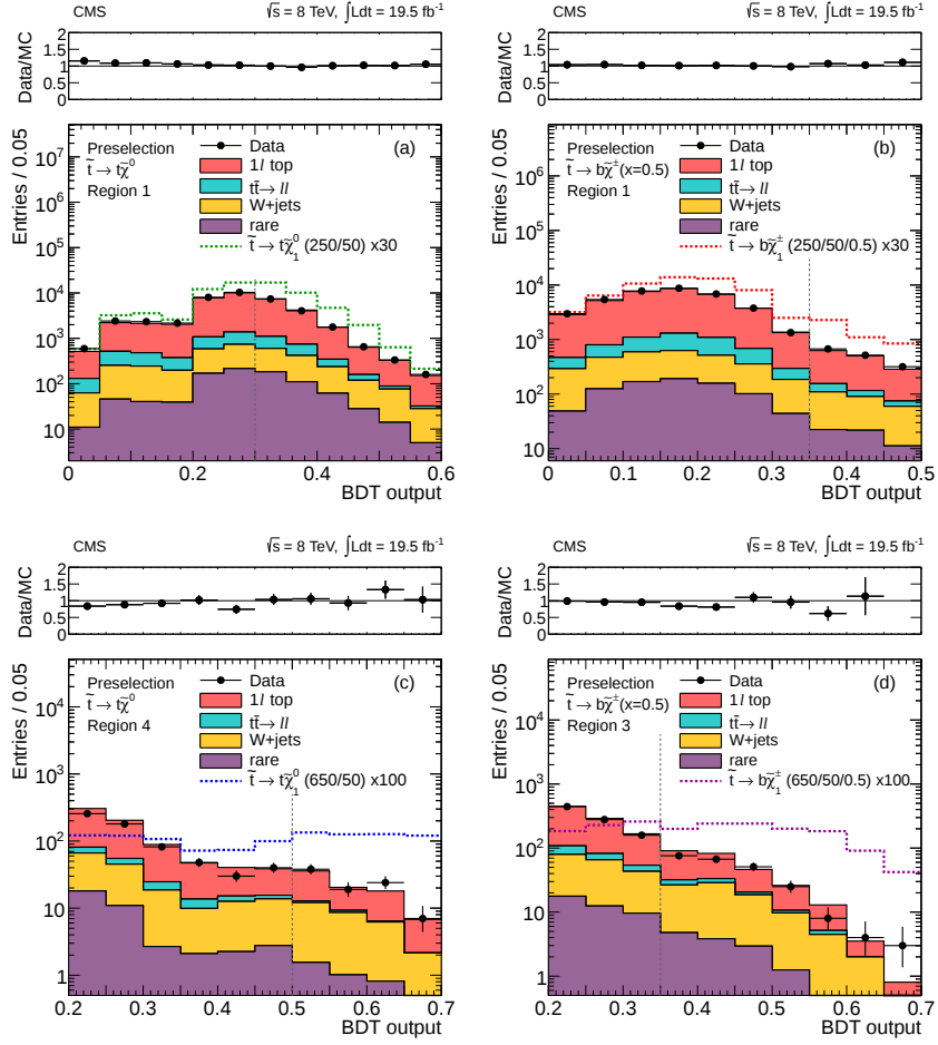
Figure 4: Comparison of data and MC simulation for sample BDT outputs. (a) \tilde{t} \rightarrow t\tilde{\chi}_1^0 scenario in training region 1; (b) \tilde{t} \rightarrow b\tilde{\chi}_1^+ scenario with x = 0.5 in training region 1; (c) \tilde{t} \rightarrow t\tilde{\chi}_1^0 scenario in training region 4; (d) \tilde{t} \rightarrow b\tilde{\chi}_1^+ scenario with x = 0.5 in training region 3. Only the event preselection is applied, and in all cases the last bin contains the overflow. Events in the signal regions are further selected by requiring M_T > 120 GeV and by applying BDT requirements as indicated by the vertical dashed lines. We also overlay expectations for possible signals with m_{\tilde{t}} = 250 GeV and m_{\tilde{\chi}_1^0} = 50 GeV (panels (a) and (b)) and m_{\tilde{t}} = 650 GeV and m_{\tilde{\chi}_1^0} = 50 GeV (panels (c) and (d)). For display purposes, these are scaled up by factors of 30 and 100 respectively.
