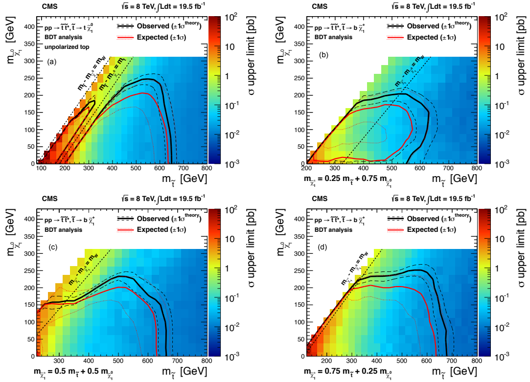
Figure 10: Interpretations using the primary results from the BDT method. (a) \tilde{t} \rightarrow t\tilde{\chi}_1^0 model; (b) \tilde{t} \rightarrow b\tilde{\chi}_1^+ model with x = 0.25 ; (c) \tilde{t} \rightarrow b\tilde{\chi}_1^+ model with x = 0.50 ; (d) \tilde{t} \rightarrow b\tilde{\chi}_1^+ model with x = 0.75 ; The color scale indicates the observed cross section upper limit. The observed, median expected, and \pm 1 standard deviation ( \sigma ) expected 95% CL exclusion contours are indicated. The variations in the excluded region due to \pm 1\sigma uncertainty of the theoretical prediction of the cross section for top-squark pair production are also indicated.
