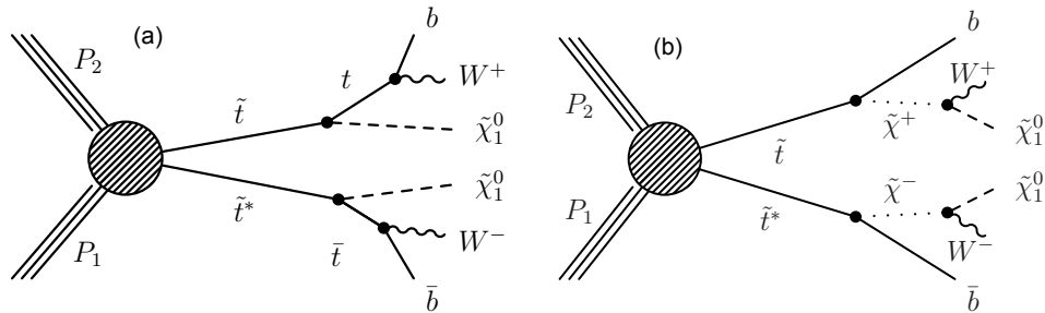
Figure 1: Diagram for top-squark pair production for (a) the \tilde{t} \rightarrow t\tilde{\chi}_1^0 \rightarrow bW\tilde{\chi}_1^0 decay mode and (b) the \tilde{t} \rightarrow b\tilde{\chi}_1^+ \rightarrow bW\tilde{\chi}_1^0 decay mode.
