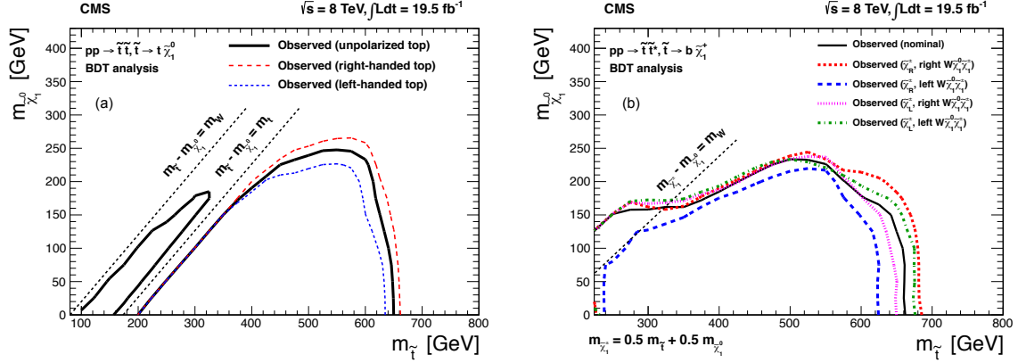
Figure 11: (a) the observed 95% CL excluded regions for the \tilde{t} \rightarrow t \tilde{\chi}_1^0 model for the case of unpolarized, right-handed, and left-handed top quarks. (b) the observed 95% CL excluded regions for the \tilde{t} \rightarrow b \tilde{\chi}_1^+ model with x = 0.5 for the nominal scenario, right- vs. left-handed charginos ( \tilde{\chi}_R^\pm and \tilde{\chi}_L^\pm , respectively), and right- vs. left-handed W \tilde{\chi}_1^\pm \tilde{\chi}_1^\pm couplings.
