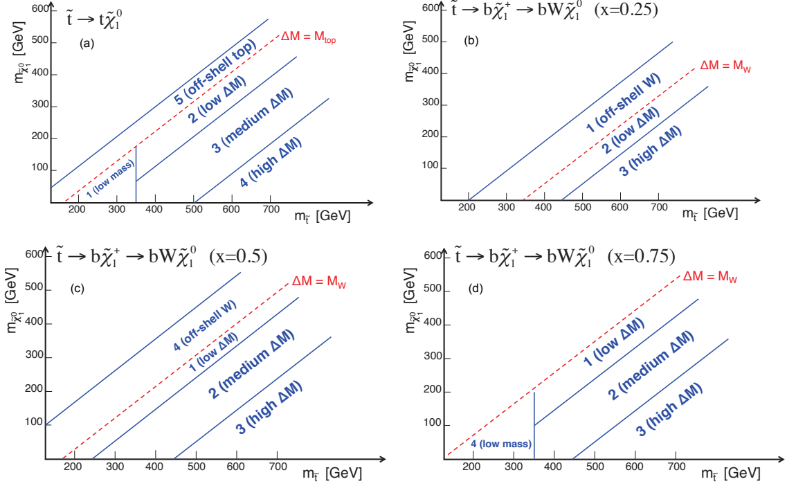
Figure 3: The regions used to train the BDTs, in the m_{\tilde{\chi}_1^0} vs. m_{\tilde{t}} parameter space, for (a) the \tilde{t} \rightarrow t\tilde{\chi}_1^0 scenario, and for (b) the \tilde{t} \rightarrow b\tilde{\chi}_1^+ x = 0.25 , (c) 0.5, and (d) 0.75 scenarios. The dashed lines correspond to \Delta M \equiv m_{\tilde{t}} - m_{\tilde{\chi}_1^0} = M_{\text{top}} for \tilde{t} \rightarrow t\tilde{\chi}_1^0 , and \Delta M \equiv m_{\tilde{\chi}_1^+} - m_{\tilde{\chi}_1^0} = M_W for \tilde{t} \rightarrow b\tilde{\chi}_1^+ .
