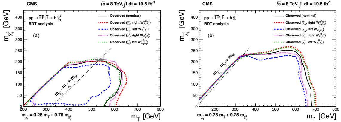
Figure 23: The observed 95% CL excluded regions for the \tilde{t} \rightarrow b\tilde{\chi}^+ model with (a) x = 0.25 and (b) 0.75 for the nominal scenario, right- vs. left-handed charginos ( \tilde{\chi}_R^\pm and \tilde{\chi}_L^\pm , respectively), and right- vs. left-handed W\tilde{\chi}_1^0\tilde{\chi}_1^\pm couplings.
