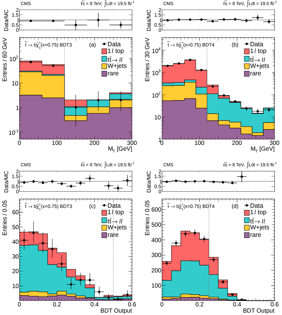
Figure 19: Comparison of data and MC simulation for the distributions of BDT output and M_T corresponding to the x = 0.75 \tilde{t} \rightarrow b\tilde{\chi}_1^+ scenario in training regions 3 and 4. The M_T distributions are shown after the requirement on the BDT output, and the BDT output distributions are shown after the M_T > 120 \text{ GeV} requirement (these requirements are also indicated by vertical dashed lines on the respective distributions). (a) M_T after the cut on the BDT3 output; (b) M_T after the cut on the BDT4 output; (c) BDT3 output after the M_T cut; (d) BDT4 output after the M_T cut. In all distributions the last bin contains the overflow.
