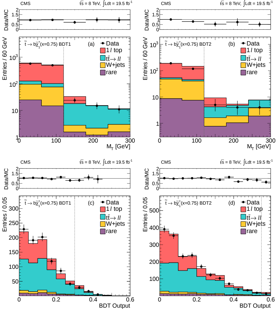
Figure 18: Comparison of data and MC simulation for the distributions of BDT output and M_T corresponding to the x = 0.75 \tilde{t} \rightarrow b\tilde{\chi}_1^+ scenario in training regions 1 and 2. The M_T distributions are shown after the requirement on the BDT output, and the BDT output distributions are shown after the M_T > 120 GeV requirement (these requirements are also indicated by vertical dashed lines on the respective distributions). (a) M_T after the cut on the BDT1 output; (b) M_T after the cut on the BDT2 output; (c) BDT1 output after the M_T cut; (d) BDT2 output after the M_T cut. In all distributions the last bin contains the overflow.
