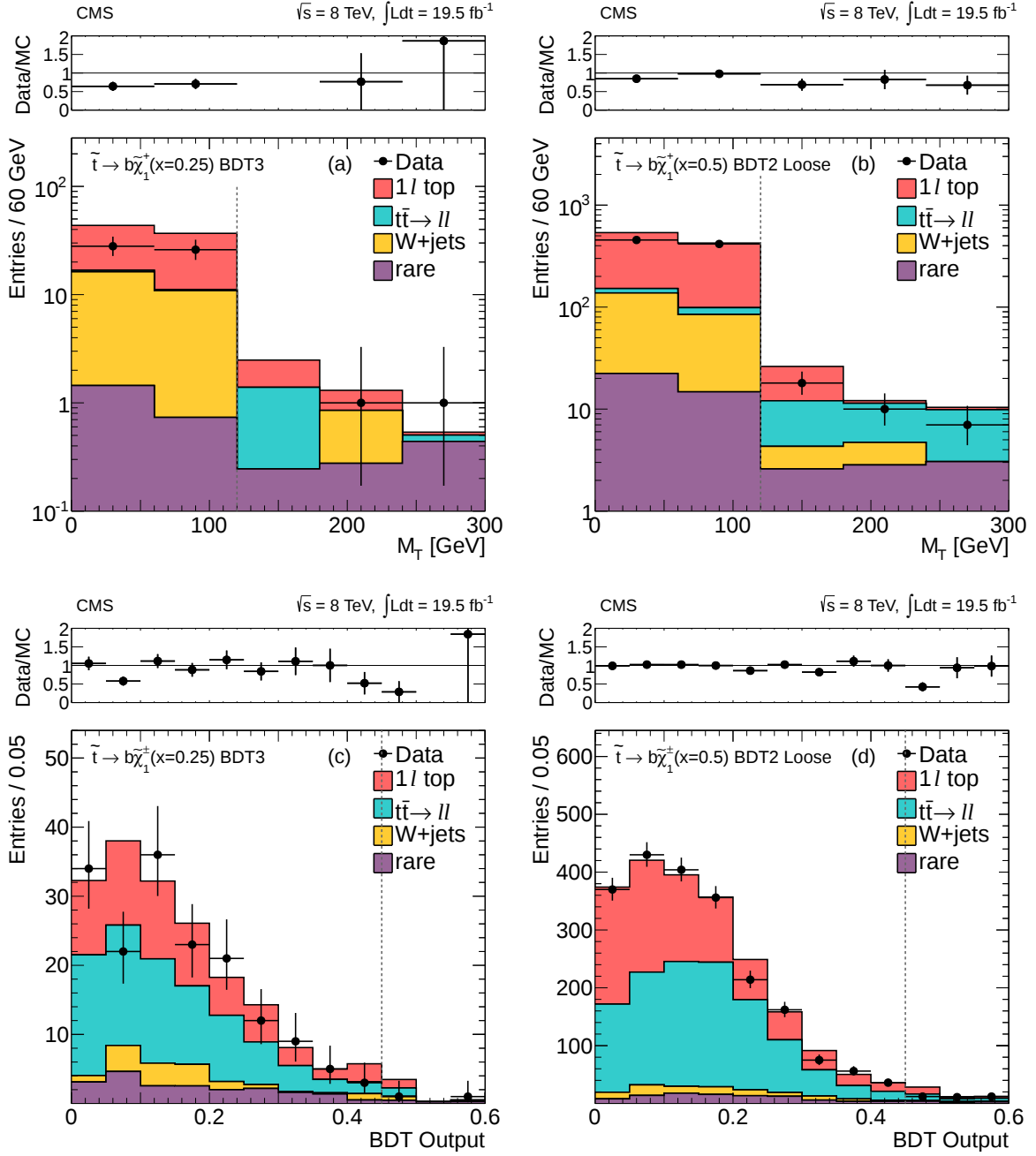
Figure 16: Comparison of data and MC simulation for the distributions of BDT output and M_T corresponding to the \tilde{t} \rightarrow b\tilde{\chi}_1^+ scenario in training regions 3 (for x = 0.25 ) and 2 (for x = 0.5 ). The M_T distributions are shown after the requirement on the BDT output, and the BDT output distributions are shown after the M_T > 120 GeV requirement (these requirements are also indicated by vertical dashed lines on the respective distributions). (a) M_T after the cut on the BDT3 ( x = 0.25 ) output; (b) M_T after the loose cut on the BDT2 ( x = 0.5 ) output; (c) BDT3 ( x = 0.25 ) output after the M_T cut; (d) BDT2 ( x = 0.5 ) output after the M_T cut. In all distributions the last bin contains the overflow.
