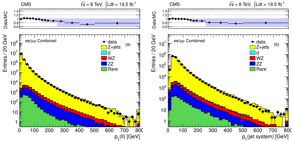
Figure 24: Comparison of data to MC predictions for the (a) dilepton p_T and (b) jet recoil system p_T in Z + jets events. The MC prediction is normalized to the total data yield. The data/MC ratio is also shown. The shaded band is centered on the weight values. The width of the band indicates the associated systematic uncertainty. In both distributions the last bin contains the overflow.
