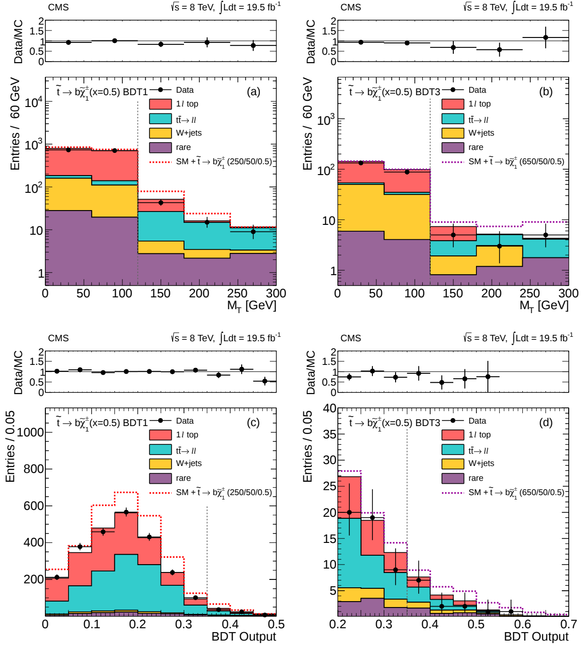
Figure 9: Comparison of data and MC simulation for the distributions of BDT output and M_T corresponding to the tightest and loosest signal region selections in the x = 0.5 \tilde{t} \rightarrow b\tilde{\chi}_1^+ scenario with an on-shell W boson. The M_T distributions are shown after the requirement on the BDT output, and the BDT output distributions are shown after the M_T > 120 GeV requirement (these requirements are also indicated by vertical dashed lines on the respective distributions). (a) M_T after the cut on the BDT1 output; (b) M_T after the cut on the BDT3 output; (c) BDT1 output after the M_T cut; (d) BDT3 output after the M_T cut. Expected signal distributions for x = 0.5 with m_{\tilde{\chi}_1^0} = 50 GeV and m_{\tilde{t}} = 250 GeV or 650 GeV are also overlayed, as indicated in the figures. In all distributions the last bin contains the overflow.
