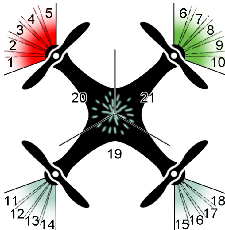
Figure 3.7: Configuration of Position and Anti-Collision on Quadcopter (1,2,3,4,5 - Left Position Light; 6,7,8,9,10 - Right Position Light; 11,12,13,14,15,16,17,18 - Rear Position Light; 19,20,21 - Anti-Collision Light)
