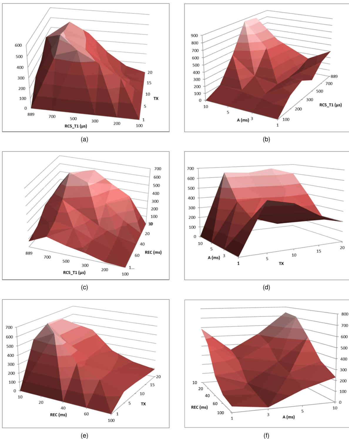
Figure 5.3: Results with relations between variables (lighter colors is better): (a) relation between 'TX' and 'RC5_T1'; (b) relation between 'A' and 'RC5_T1'; (c) relation between 'REC' and 'RC5_T1'; (d) relation between 'TX' and 'A'; (e) relation between 'TX' and 'REC'; and, (f) relation between 'A' and 'REC'.
