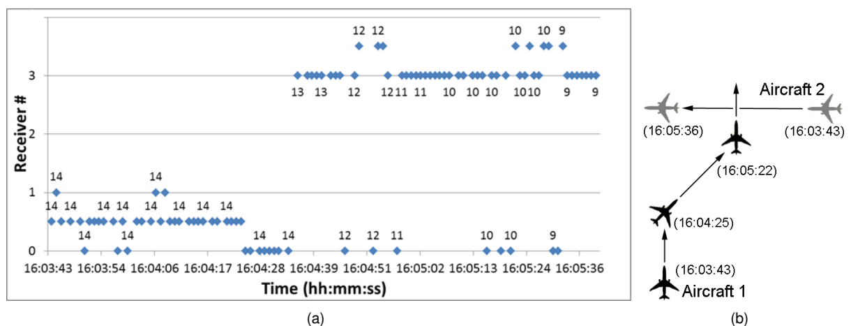
Figure 5.6: Results for converging collision avoidance maneuver: (a) Graphic with received information; and, (b) Diagram of relevant positions and respective time.
