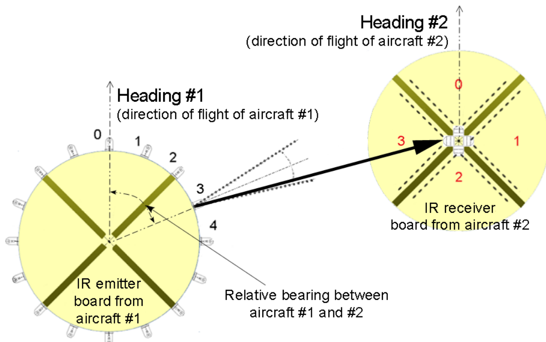
Figure 4.3: Diagram of communication between two prototypes
