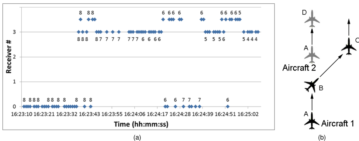
Figure 5.7: Results for overtaking collision avoidance maneuver: (a) Graphic with received information; and, (b) Diagram of relevant positions and respective time.
