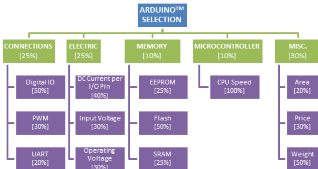
Figure 3.2: AHP study hierarchy and criteria relative weights
