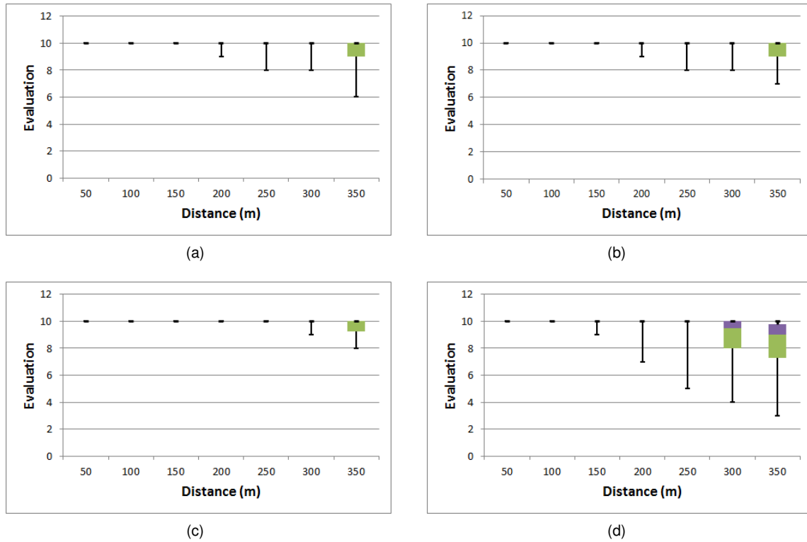
Figure 5.1: Analysis of results for each light: (a) left position; (b) right position; (c) rear position; and, (d) anti-collision.
