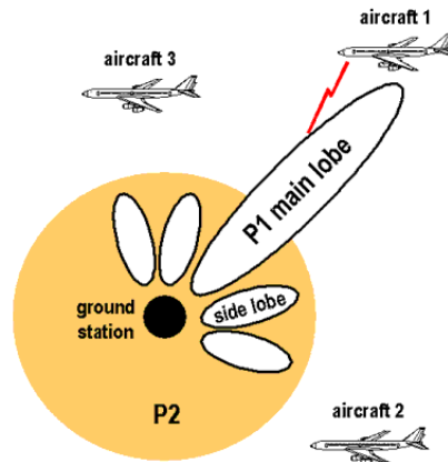
Figure 2.6: ATCRBS Broadcast with Omnidirectional Antenna [10]
