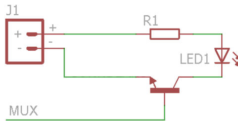
Figure 4.9: Diagram of the TSAL6100 and the ULN2803A Array connections - the array is simplified into a single transistor
