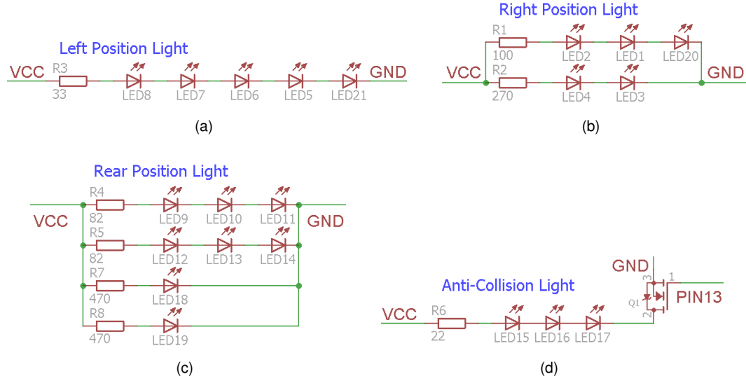
Figure 3.3: Schematic Diagram of each Light: (a) describes the Left Position Light; (b) describes the Right Position Light; (c) describes the Rear Position Light; and, (d) describes the Anti-Collision Light.
