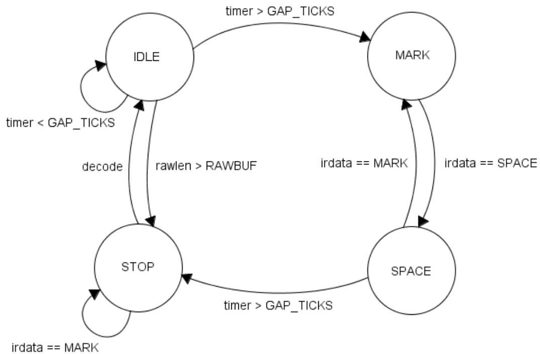
Figure 4.12: IRremote Reception Space State
