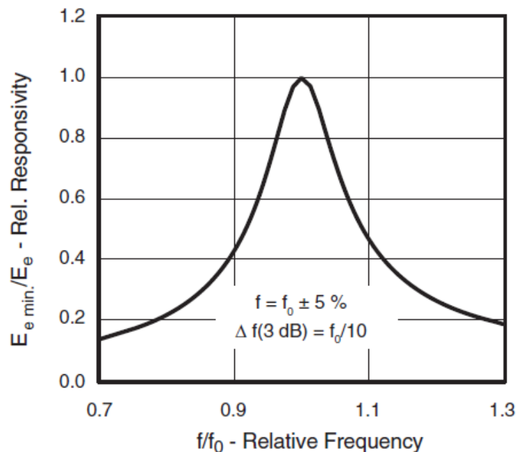
Figure 4.5: IR Receiver TSOP48's Frequency Dependence of Responsivity [25]
