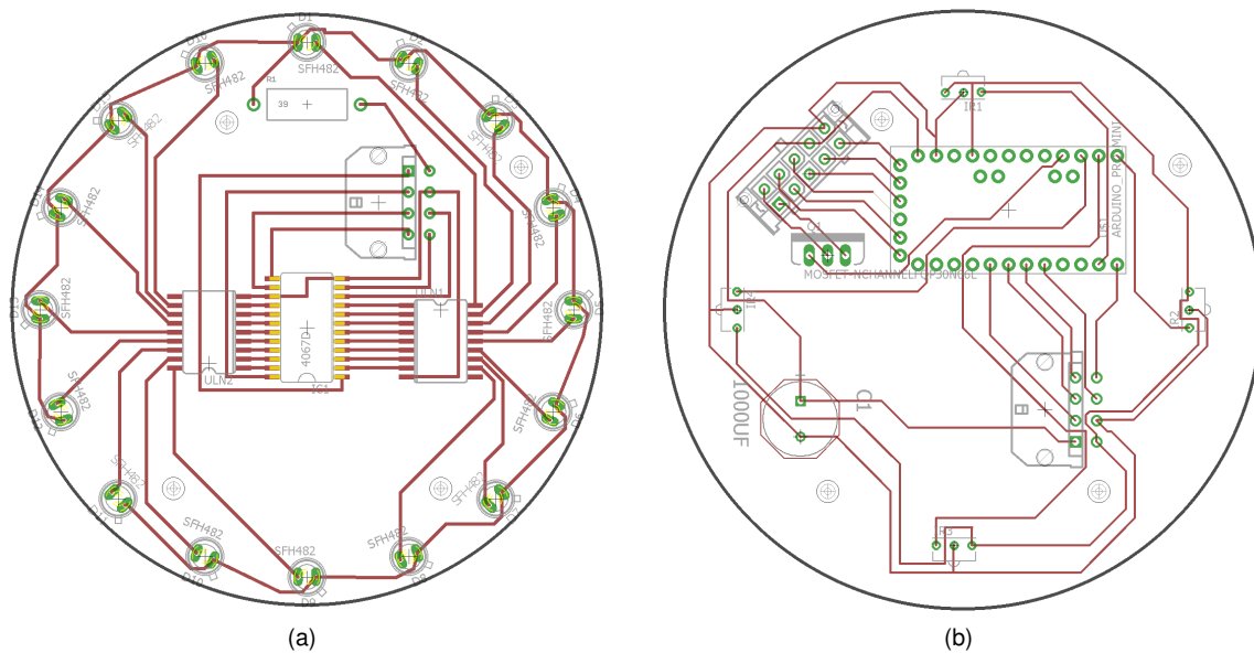
Figure 4.16: Second Prototype: (a) transmitter board; and, (b) receiver board.
