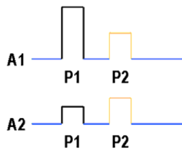
Figure 2.7: ATCRBS Broadcast Pulses (A1 - aircraft 1; A2 - aircraft 2) [10]
