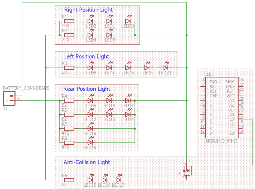
Figure 3.8: Schematic for Position and Anti-Collision Light System
