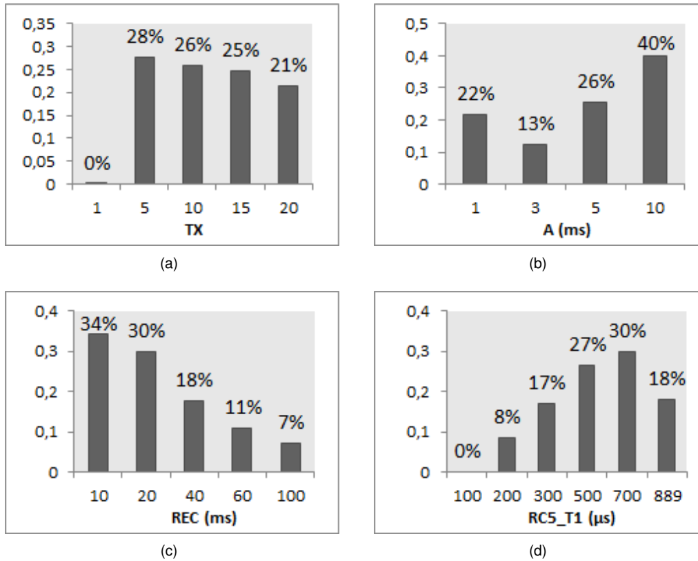
Figure 5.2: Number of receptions for each variable (higher is better): (a) 'TX'; (b) 'A'; (c) 'REC'; and, (d) 'RC5_T1'.
