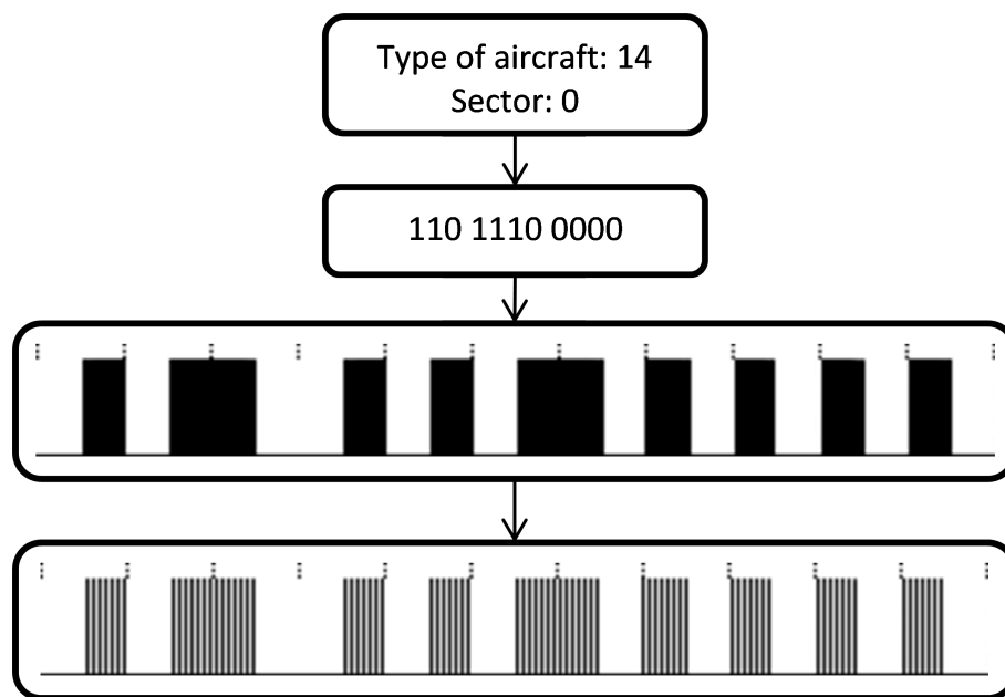
Figure 4.11: Process of Modulating the Transmitted Message - signal not to scale
