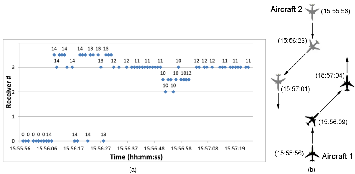
Figure 5.5: Results for head-on collision avoidance maneuver: (a) Graphic with received information; and, (b) Diagram of relevant positions and respective time.
