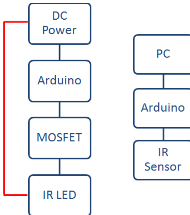
Figure 2. Block diagram of the IR Anti-Collision Subsystems for the Test
