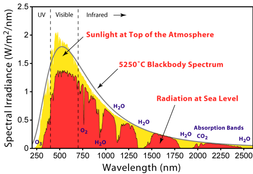
Figure 4.2: Solar Radiation Spectrum [23]
