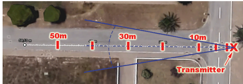
Figure 4.13: Distances and Positions for both Subsystems for range and receiver's field coverage tests
