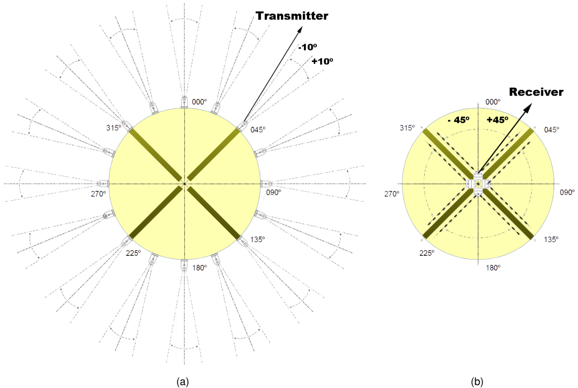
Figure 4.6: Diagram of IR boards: (a) emitter board; and, (b) receiver board.
