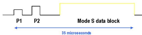
Figure 2.8: Mode S Signal with Sidelobe Suppression [10]
