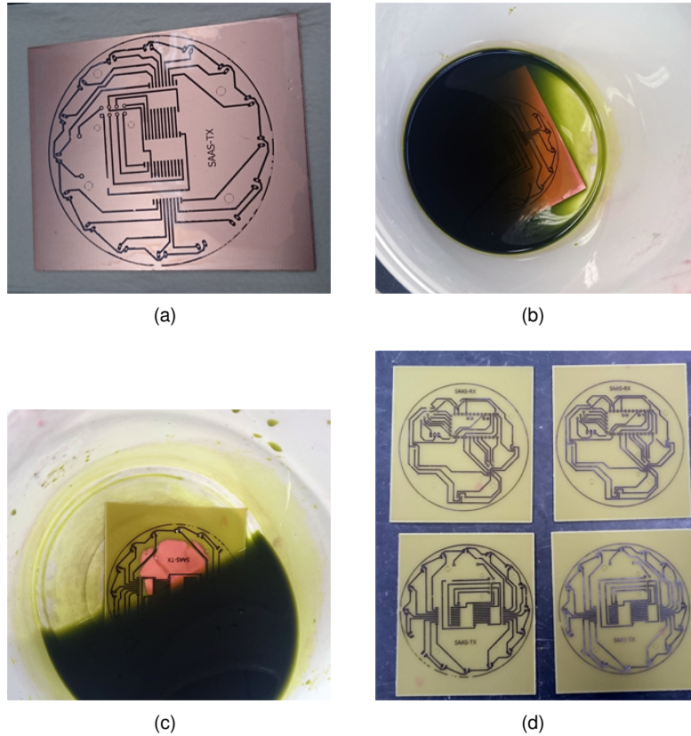
Figure 4.17: PCB printing process: (a) printed image transferred to copper; (b) iron chloride reacting with copper; (c) iron chloride reacting with copper; and, (d) finished boards.
