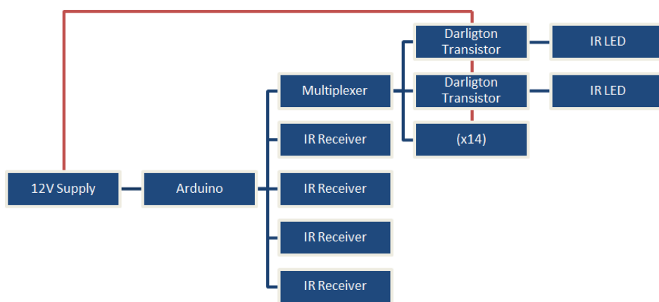
Figure 4.7: Block Diagram of the IR Anti-Collision System
