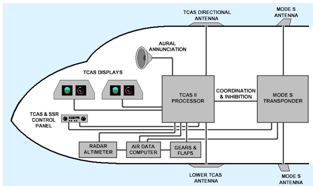
Figure 2.10: Block diagram of TCAS and transponder hardware components required for standard TCAS equipment [12]
