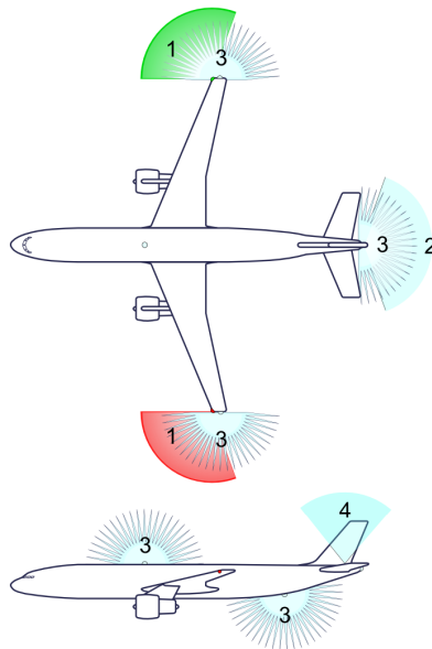
Figure 2.5: Aviation Lights used in See and Avoid. 1) Left and Right Position Lights; 2) Rear Position Light; 3) Anti-collision Lights; 4) Logo Light; [11]
