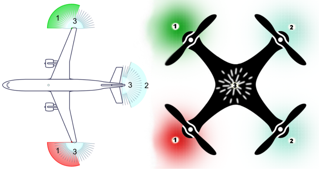
Figure 3.1: Configuration of Position and Anti-Collision for Two Different Aircraft (1-left and right position lights; 2-rear position lights; 3-anti-collision lights)
