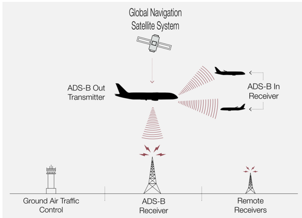
Figure 2.11: ADS-B communications [13]
