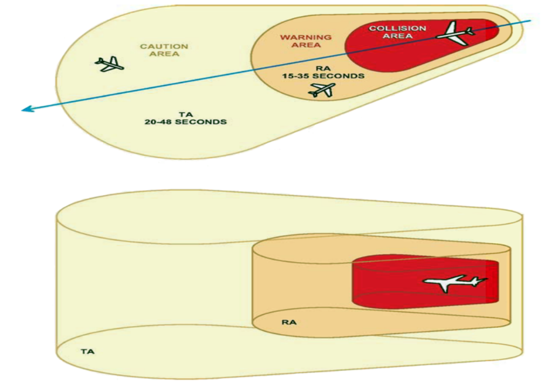
Figure 2.9: TCAS Protection Volume - Not to scale [2]
