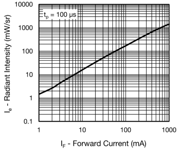
Figure 4.8: TSAL6100 Radiant Intensity vs. Forward Current [26]
