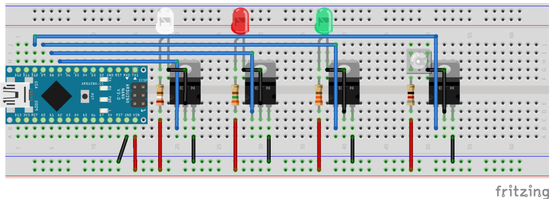
Figure 9. Diagram for the test procedure
