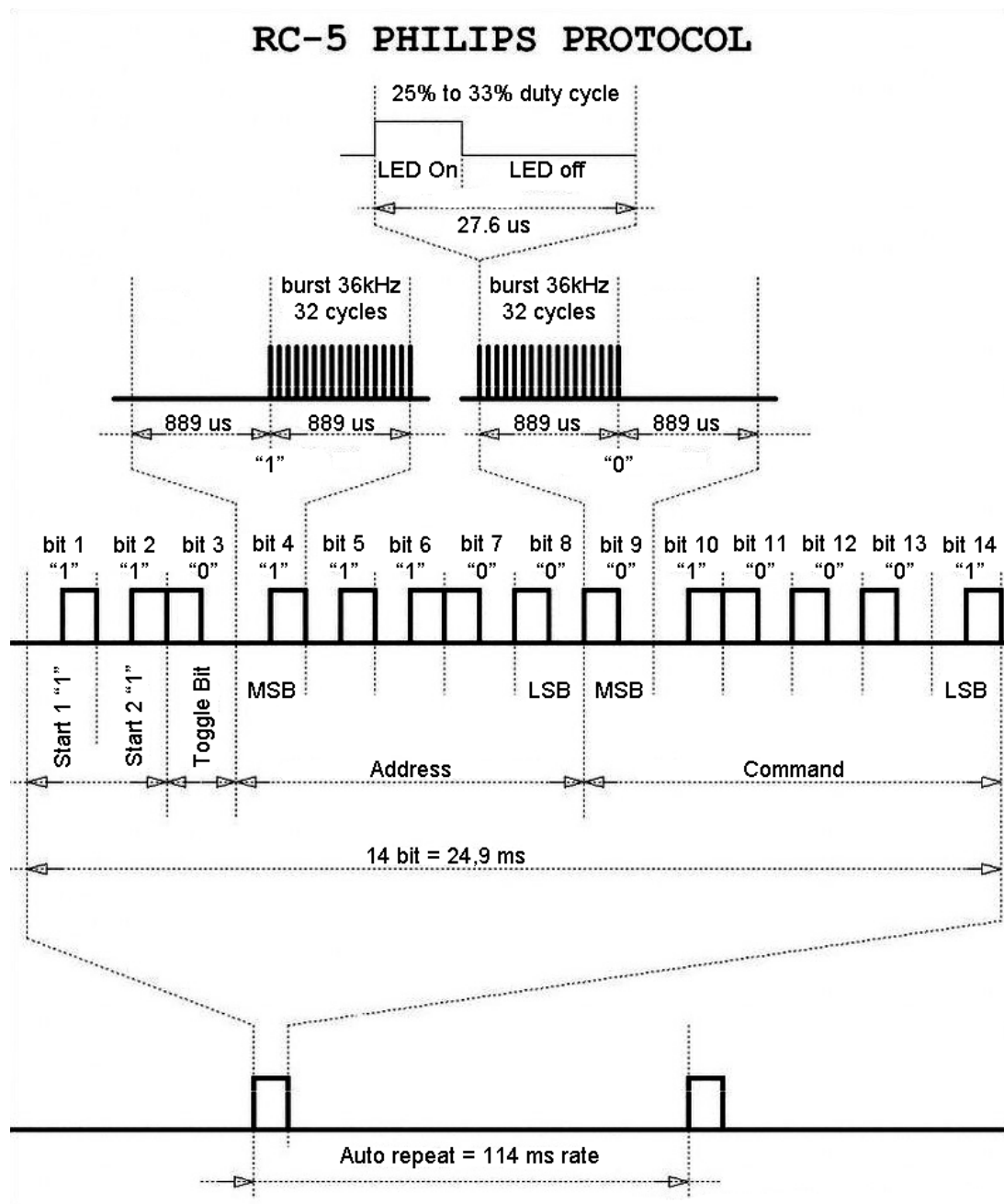
Figure 4.4: RC5-5 Philips Protocol details [24]
