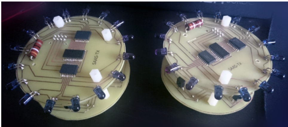
Figure 4.18: Finished prototypes
