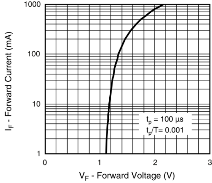
Figure 4.10: TSAL6100 Forward Current vs Forward Voltage [26]
