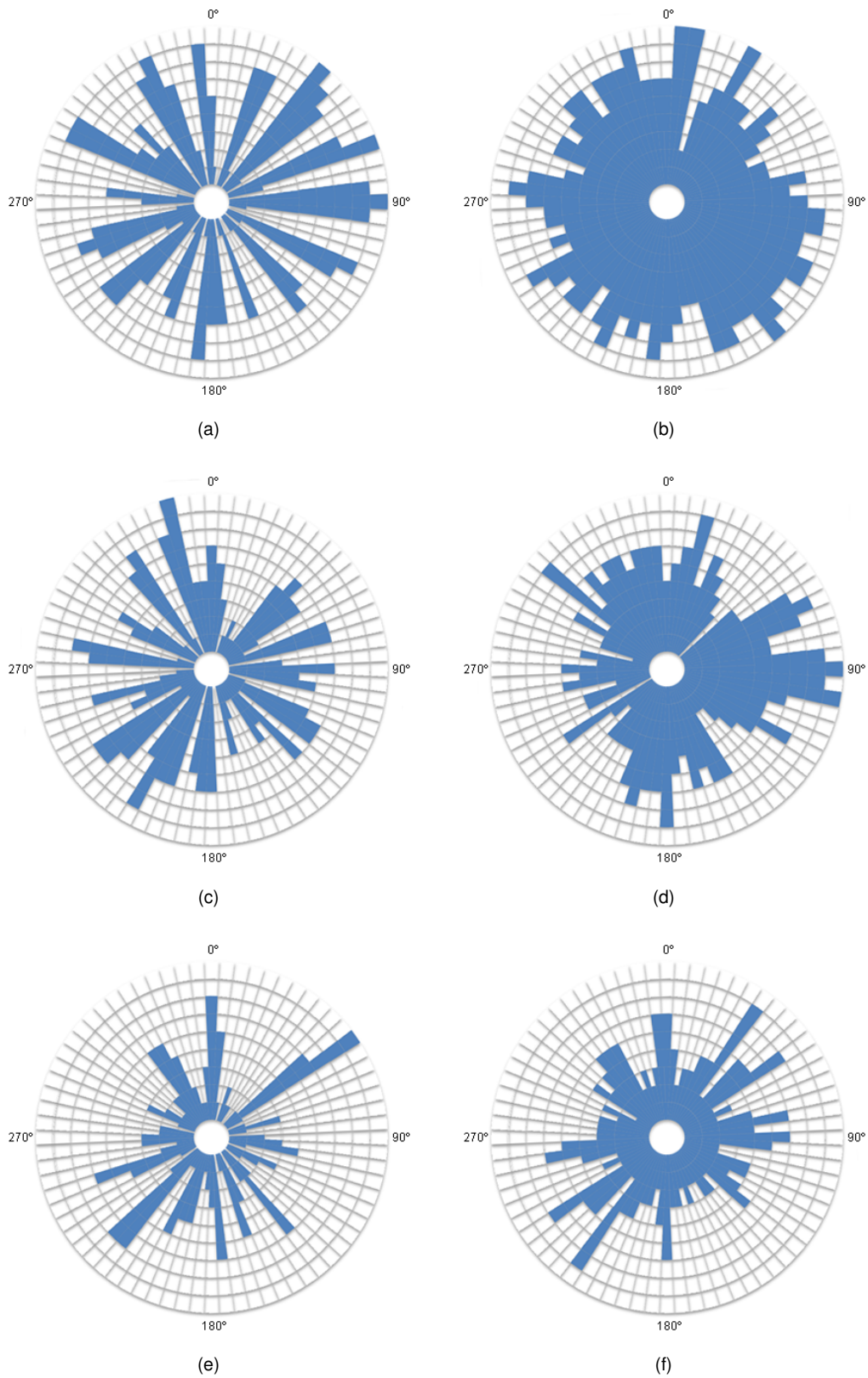
Figure 5.4: Number of receptions for each 5° sector (higher is better): (a) transmission at 14 m; (b) reception at 14 m; (c) transmission at 18 m; (d) reception at 18 m; (e) transmission at 22 m; and, (f) reception at 22 m.
