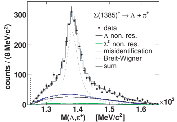
FIG. 7: Color online. Invariant mass distribution of the selected \Lambda - \pi^+ pairs. The circles show the experimental data, the black and green curves depict the contributions coming from the non-resonant production, the blue curve shows the misidentification background and the gray dashed curve represents a Breit-Wigner distribution fitted to the data. The solid gray histogram represents the result of the final fit (see text for details). Dashed vertical lines depict the interval chosen for the fit.
