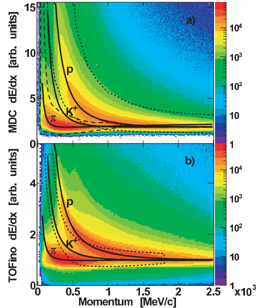
FIG. 1: Color online. dE/dx versus momentum for all detected particles in the MDC (panel (a)) and TOFino (panel (b)) detectors. The solid black curves indicate adapted Bethe-Bloch formulas and the dashed ones show the interval used to select protons and pions in the MDC (panel (a)) and kaons in TOFino (panel (b)).
