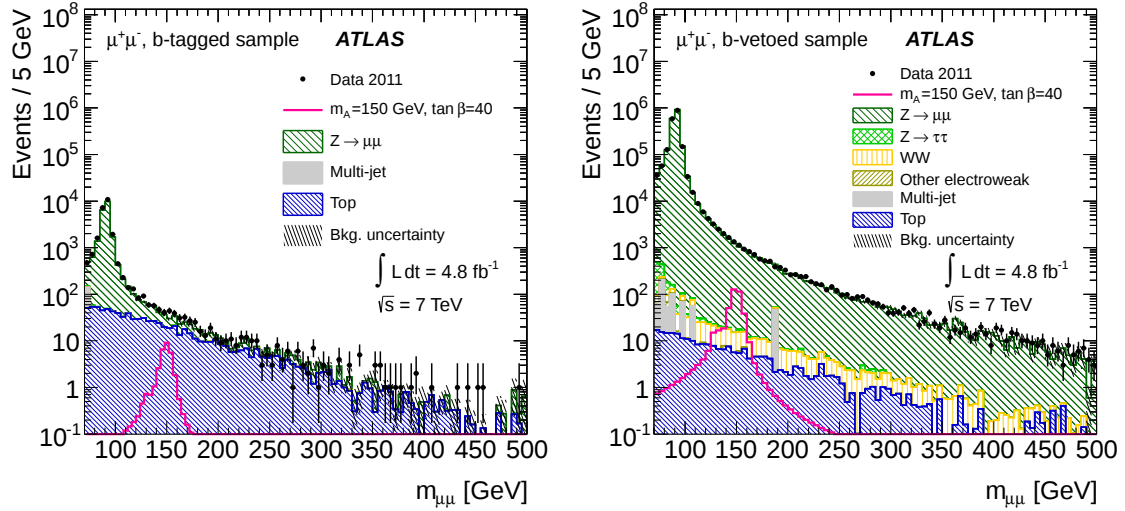
Figure 1. The invariant mass distribution of the two muons of the h/A/H \rightarrow \mu^+\mu^- search for the b -tagged (left-hand side) and the b -vetoed samples (right-hand side). The data are compared to the background expectation and a hypothetical MSSM signal ( m_A = 150 GeV, \tan\beta = 40 ). Simulated backgrounds are shown for illustration purposes. The background uncertainties shown here are statistical in nature due to the finite number of simulated events. The contributions of the backgrounds Z/\gamma^* \rightarrow e^+e^- , W + \text{jets} and those of all diboson production processes but WW production are combined and labelled “Other electroweak”.
