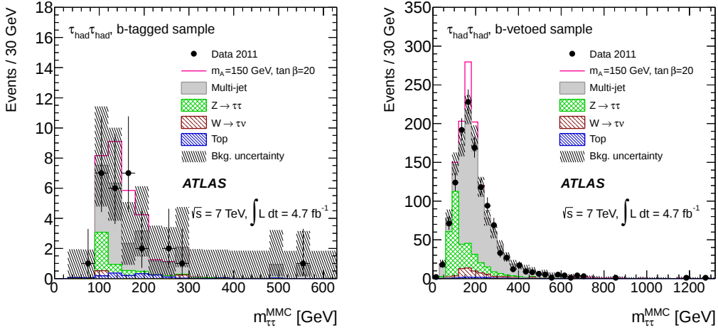
Figure 5. MMC mass distributions for the h/A/H \rightarrow \tau_{\text{had}}\tau_{\text{had}} final state. The MMC mass, m_{\tau\tau}^{\text{MMC}} , is shown for the b -tagged (left-hand side) and b -vetoed samples (right-hand side). The data are compared to the background expectation and an added hypothetical MSSM signal ( m_A = 150 GeV and \tan \beta = 20 ). The background uncertainties include statistical and systematic uncertainties.
