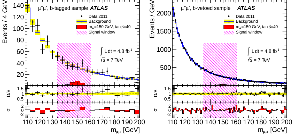
Figure 2. Invariant mass distribution of data and predicted background from sideband fits to the data shown for the signal mass point at m_A = 150 GeV and \tan \beta = 40 for the b -tagged (left-hand side) and the b -vetoed samples (right-hand side) of the h/A/H \rightarrow \mu^+\mu^- final state. The ratio of the data to the predicted background, labelled D/B , and the bin-by-bin significances of the deviations of the data from the background prediction, labelled \sigma , are shown beneath.
