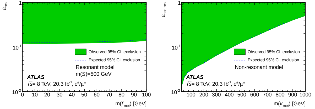
Fig. 7. Observed and expected excluded coupling strengths (left) for the resonant model with m(S) = 500 GeV and (right) for the non-resonant model, as a function of the mass of f_{\text{met}} and \nu_{\text{met}} , respectively.
