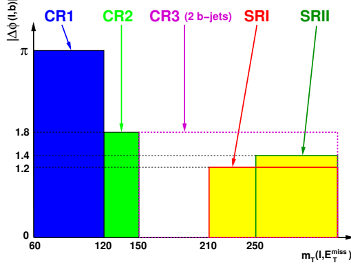
Fig. 3. Sketch depicting the control and signal regions in the (m_T(\ell, E_T^{\text{miss}}), |\Delta\phi(\ell, b)|) -space. The CR1 (CR2) control region is defined as 60 \text{ GeV} < m_T(\ell, E_T^{\text{miss}}) < 120 \text{ GeV} ( 120 \text{ GeV} < m_T(\ell, E_T^{\text{miss}}) < 150 \text{ GeV} and |\Delta\phi(\ell, b)| < 1.8 ). The CR3 control region corresponds to m_T(\ell, E_T^{\text{miss}}) > 150 \text{ GeV} and |\Delta\phi(\ell, b)| < 1.8 , but with a second b -tagged jet. The SRI (SRII) signal selection optimised for the resonant (non-resonant) signal model, is defined as m_T(\ell, E_T^{\text{miss}}) > 210 \text{ GeV} and |\Delta\phi(\ell, b)| < 1.2 ( m_T(\ell, E_T^{\text{miss}}) > 250 \text{ GeV} and |\Delta\phi(\ell, b)| < 1.4 ).
