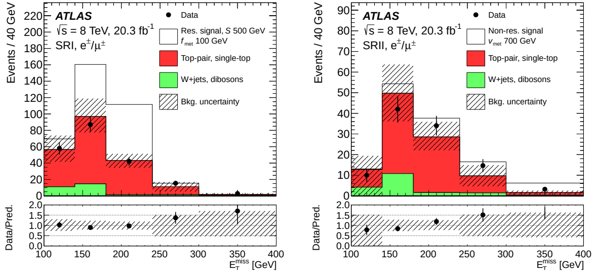
Fig. 5. Distributions of E_T^{\text{miss}} in the (left) SRI and (right) SRII signal regions, for the electron and muon channels combined. The distributions observed in data, depicted with the points, are compared with the predicted background contributions, shown stacked together with the expected resonant (non-resonant) signal contribution for the m(f_{\text{met}}) = 100 GeV and m(S) = 500 GeV ( m(v_{\text{met}}) = 700 GeV) hypothesis. The expected backgrounds are normalised to their theoretical cross-sections, and the expected resonant (non-resonant) signal is normalised to the theoretical cross-section corresponding to a_{\text{res}} = 0.2 ( a_{\text{non-res}} = 0.2 ). The error bands on the expected backgrounds correspond to the uncertainties due to all systematic sources added in quadrature. The first (last) bin includes underflows (overflows). The ratios of the observed distributions to the predicted background distributions are shown in the lower frame.
