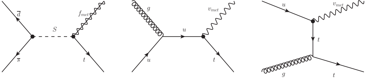
Fig. 1. Example of Feynman diagrams of leading-order processes leading to monotop events: (left) production of a coloured scalar resonance S decaying into a top quark and a spin-1/2 fermion f_{\text{met}} in the resonant model, and (middle) s - and (right) t -channel non-resonant production of a top quark in association with a spin-1 boson v_{\text{met}} in the non-resonant model.
