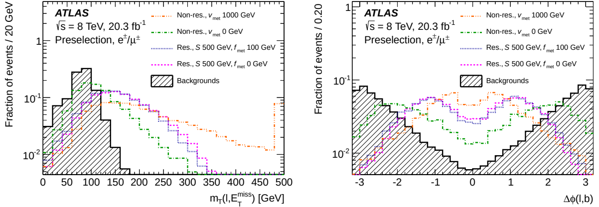
Fig. 2. Distributions normalised to unity of (left) m_T(\ell, E_T^{\text{miss}}) and of (right) \Delta\phi(\ell, b) for events satisfying the pre-selection defined in the text. The expected distributions for the resonant model with m(S) = 500 GeV are shown for the m(f_{\text{met}}) = 0 GeV and m(f_{\text{met}}) = 100 GeV hypotheses, as well as for the non-resonant model for the m(v_{\text{met}}) = 0 GeV and m(v_{\text{met}}) = 1000 GeV hypotheses. All distributions are compared to the expected distribution for the backgrounds. For the m_T(\ell, E_T^{\text{miss}}) distributions, the last bin includes overflows.
