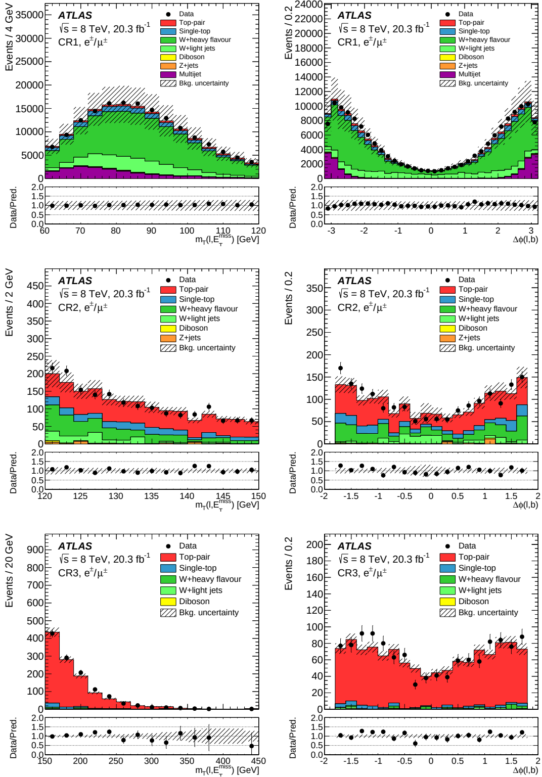
Fig. 4. Distributions of (left) m_T(\ell, E_T^{\text{miss}}) and of (right) \Delta\phi(\ell, b) in (top) the CR1, (middle) the CR2, and (bottom) the CR3 control region, for the electron and muon channels combined. The distributions observed in data, depicted with the points, are compared with the predicted background contributions. In the CR2 and CR3 regions, the negligible multijet contribution is not shown, and neither is the Z+jets contribution in the CR3 region. The multijet background is normalised by the data-driven method, and the other backgrounds are normalised to their theoretical cross-sections. The error bands correspond to the uncertainties due to the statistical uncertainty of the sample added in quadrature with a conservative 50% normalisation uncertainty on the multijet contribution, and with the W+jets and t\bar{t} cross-section uncertainties. The ratios of the observed distributions to the predicted background distributions are shown in the lower frame.
